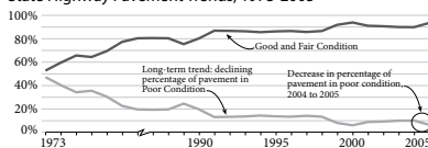
State Highway Pavement Trends, 1973-2005
