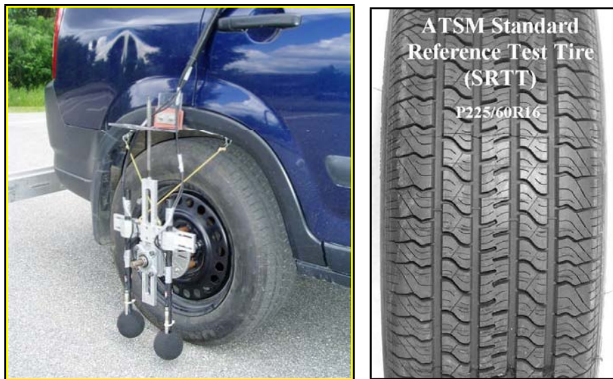
Figure 13. OBSI dual probe system and the SRTT.
