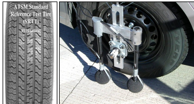
Figure 19. SI dual probe system and the SRTT.
