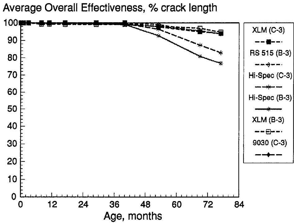
Figure 32. Time-series effectiveness trends of Des Moines, IA crack-seal treatments.
