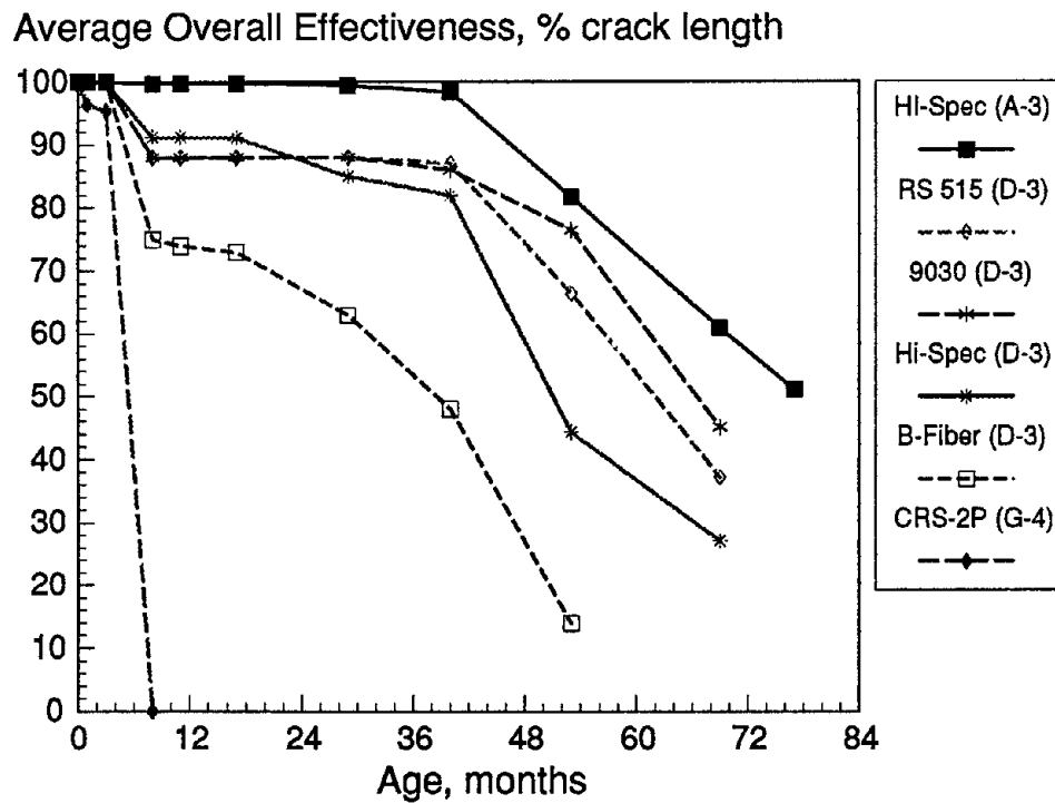
Figure 32. Time-series effectiveness trends of Des Moines, IA crack-seal treatments (continued).
