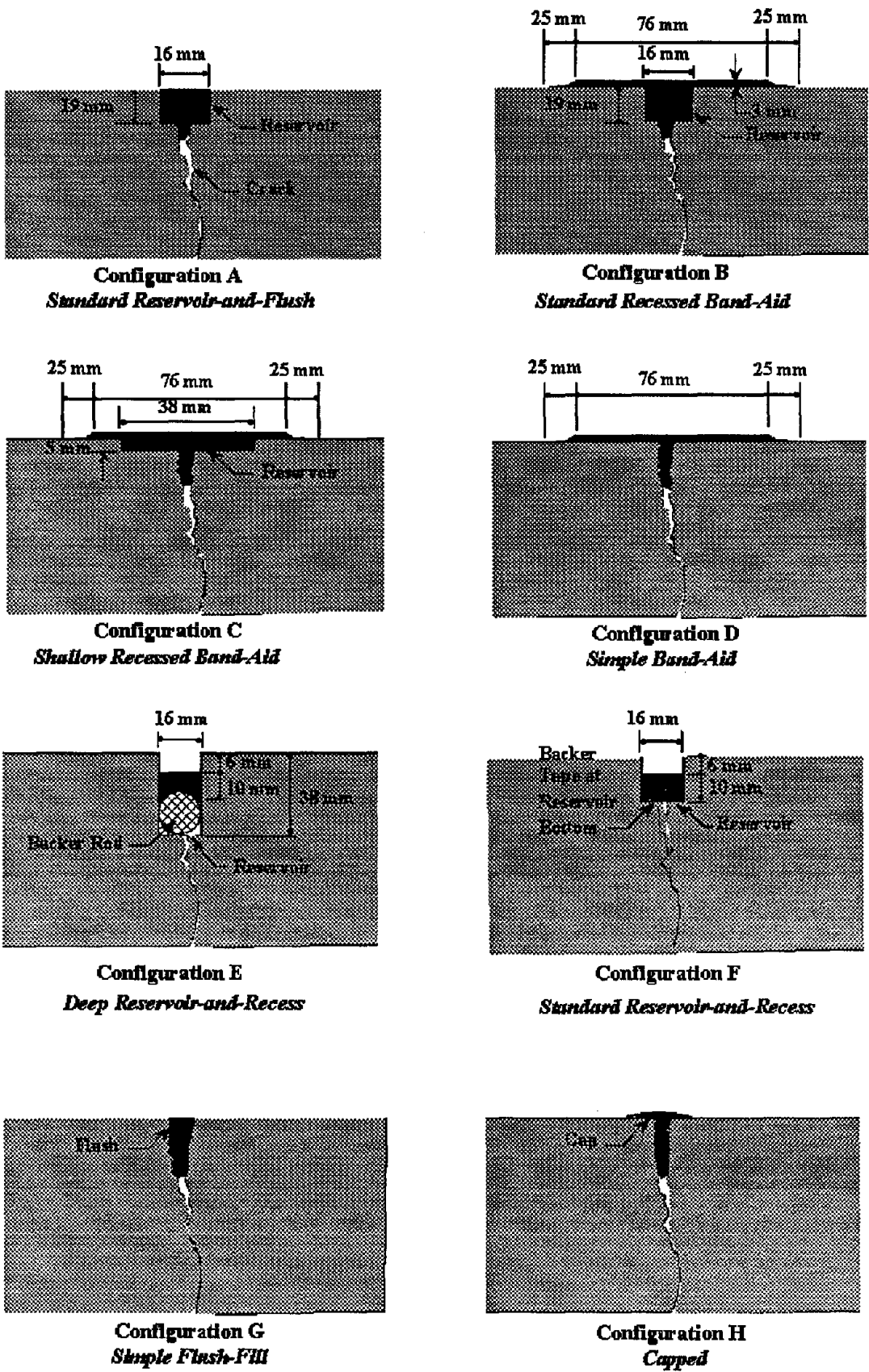
Figure 2. Material placement configurations for AC crack treatments.
