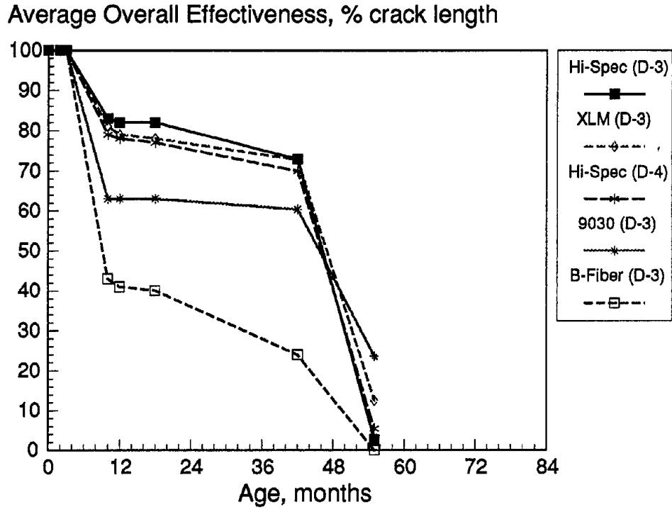
Figure 31. Time-series effectiveness trends of Wichita, KS ideal-conditions crack-seal treatments (continued).
