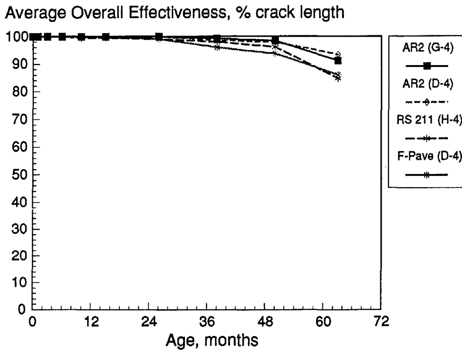
Figure 36. Time-series effectiveness trends of Prescott, ON crack-fill treatments.
