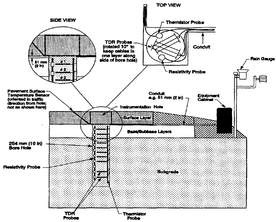
Figure 1. LTPP SMP instrumentation layout [2].
