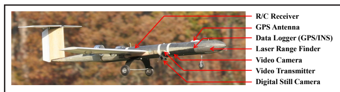
Figure 2. Aircraft Instrumentation for Remote Sensing
