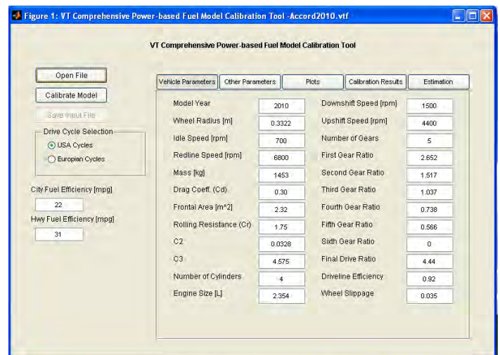
Figure 1: Illustration of CPFM Calibration Tool
