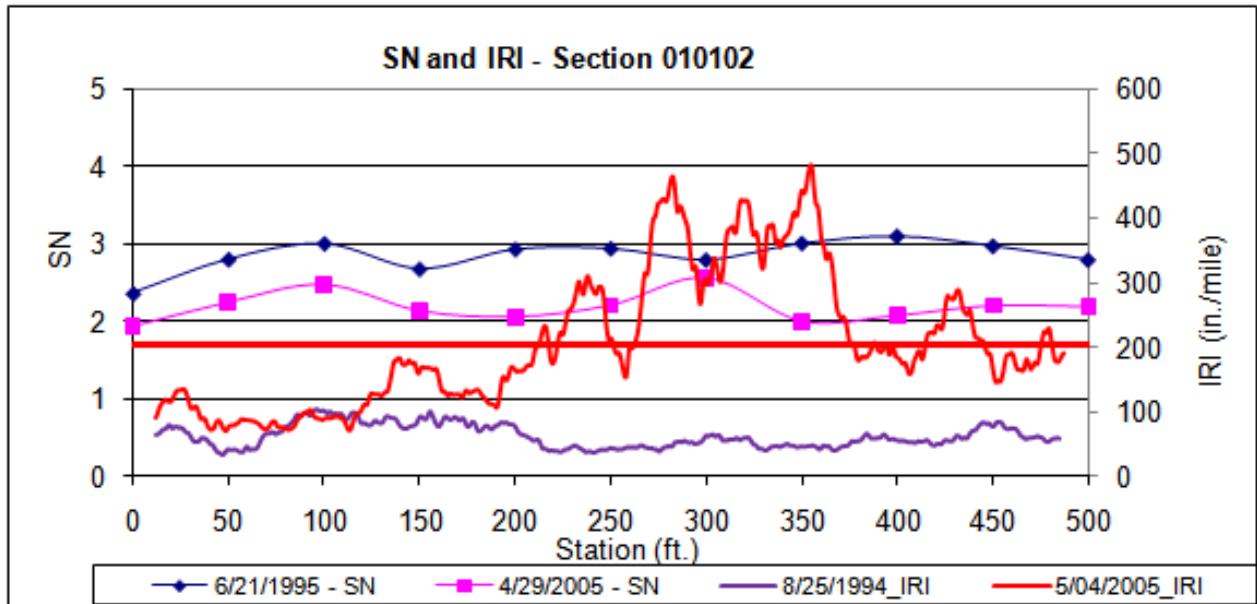
Figure 35. Graph. SN and IRI for two test dates, section 010102 (Alabama).
