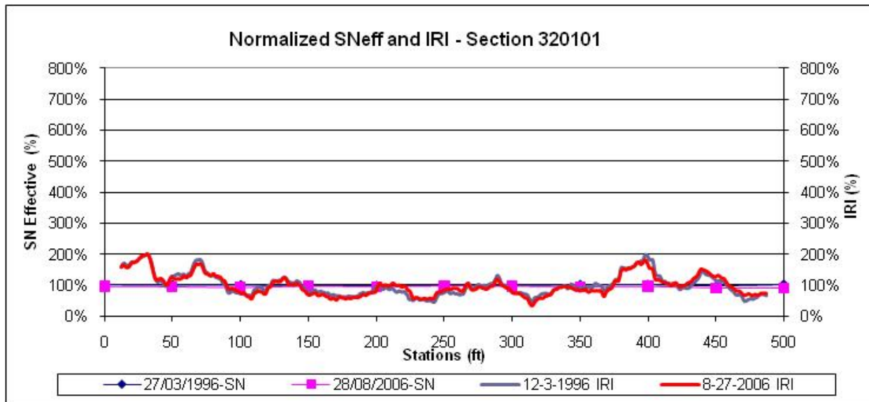
Figure 44. Graph. Normalized SN and IRI for two test dates, section 320101 (Nevada).
