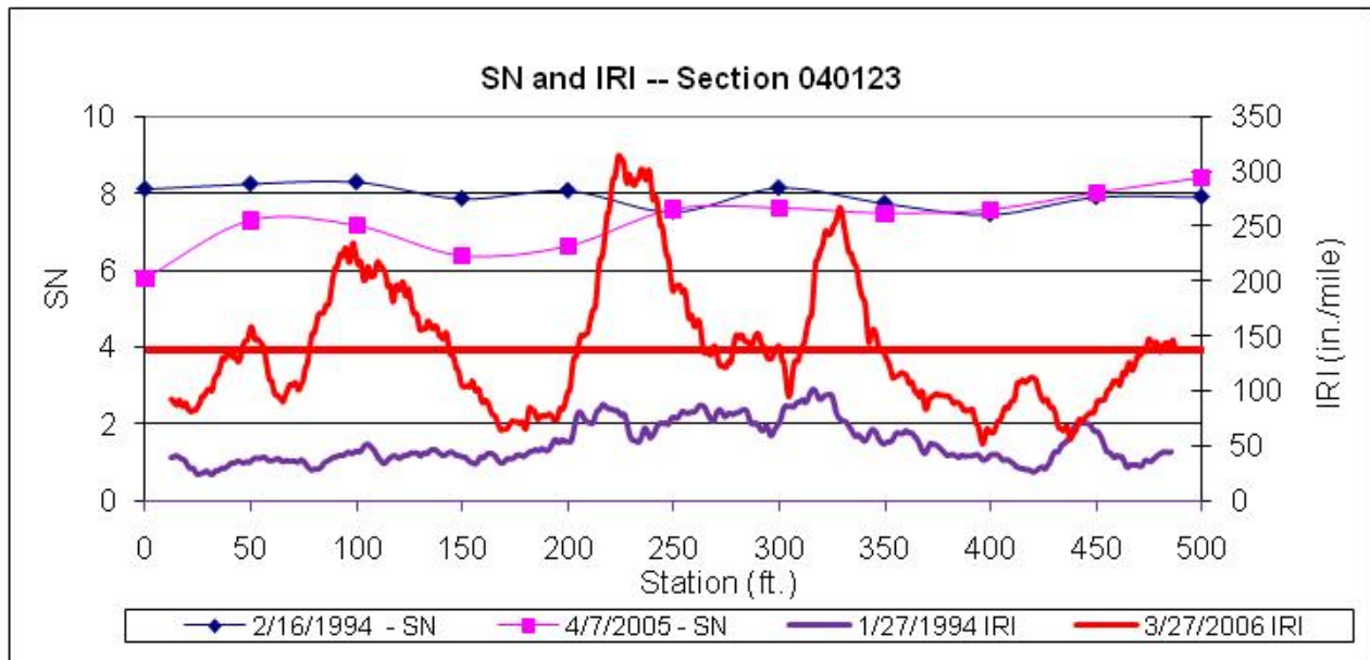
Figure 39. Graph. SN and IRI for two test dates, section 040123 (Arizona).
