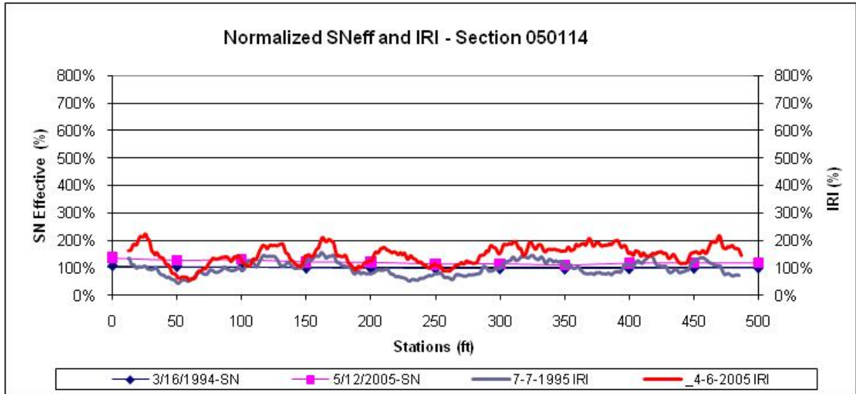
Figure 52. Graph. Normalized SN and IRI for two test dates, section 050114 (Arkansas).
