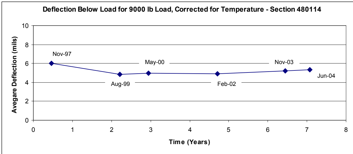
Figure 136. Graph. Average normalized deflection below 9,000-lb load, section 480114 (Texas).
