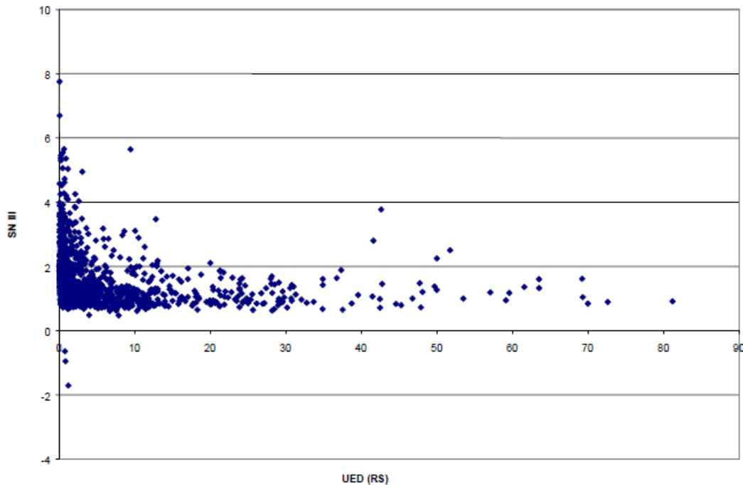
Figure 16. Graph. Sensitivity of SN to UED of ride score.
