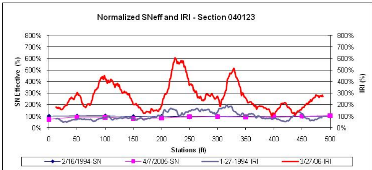
Figure 40. Graph. Normalized SN and IRI for two test dates, section 040123 (Arizona).
