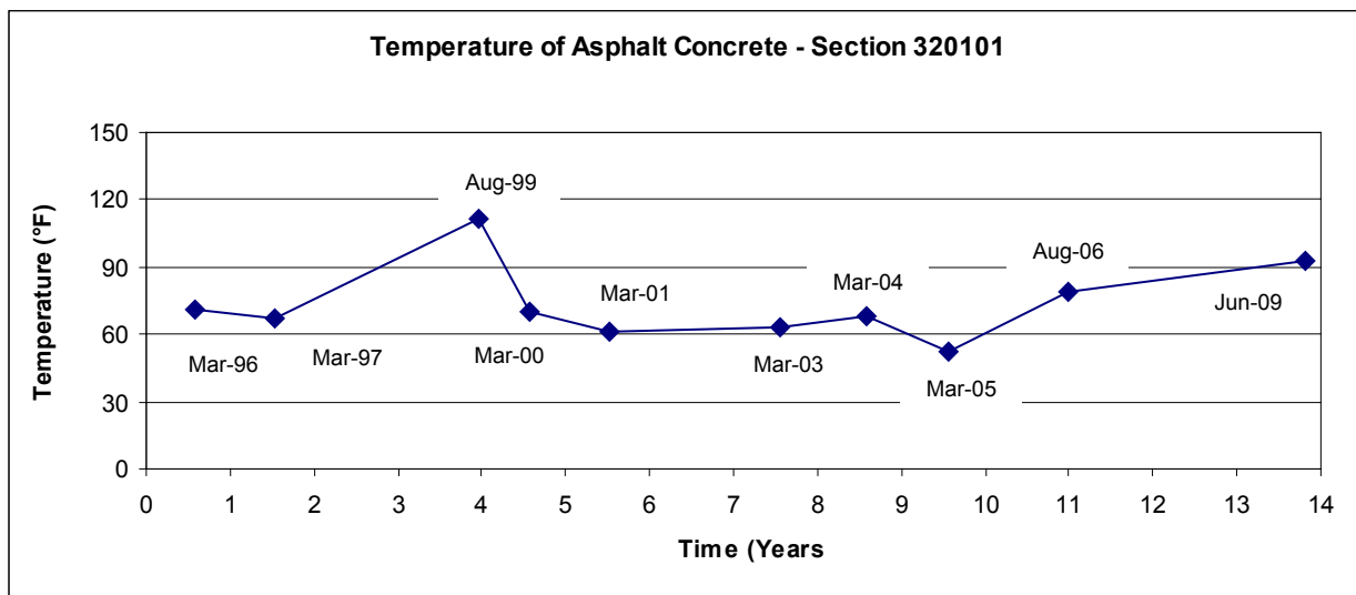
Figure 149. Graph. Mid-depth temperature of AC layer, section 320101 (Nevada).
