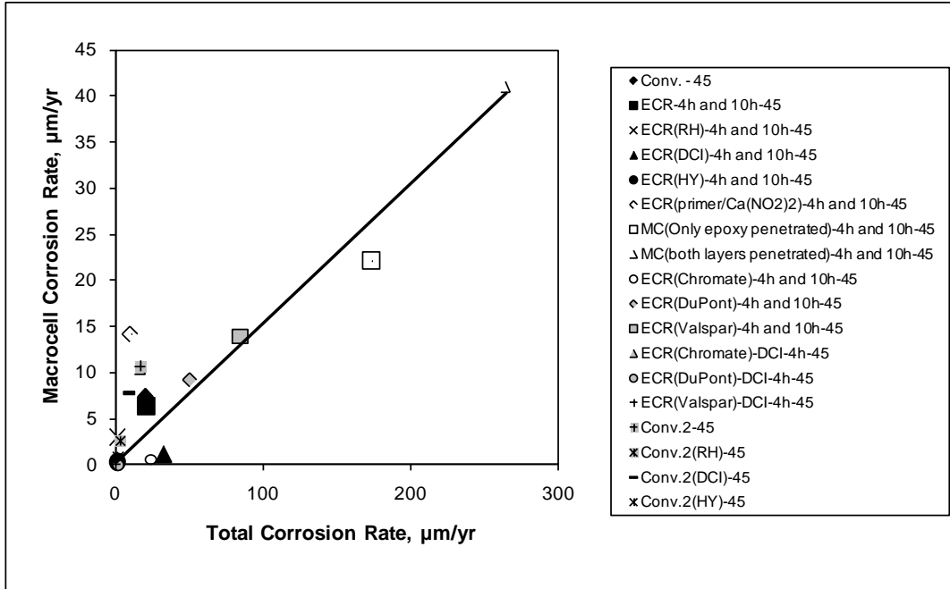
Figure 98. Graph. Southern exposure specimens, average total and macrocell corrosion rates based on losses after corrosion initiation based on total area for conventional reinforcement and area exposed at holes through coating for coated reinforcement, w/c = 0.45.
