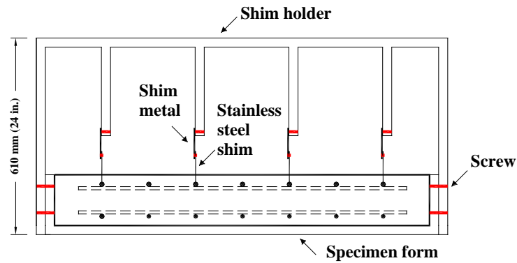
Figure 25. Illustration. Shim holder for field specimens, front view.
