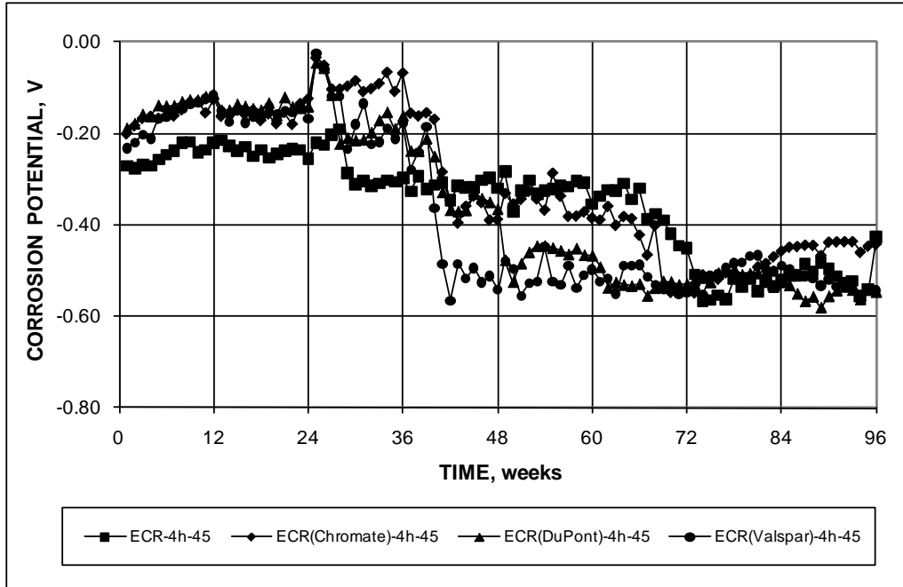
Figure 56. Graph. Southern exposure test, corrosion potential of top mat for conventional ECR and increased-adhesion ECR.
