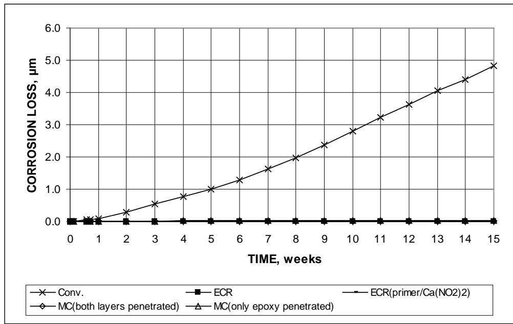
Figure 41. Graph. Macrocell test, average corrosion loss based on total area for mortar-wrapped conventional, ECR, ECR with calcium nitrite, and MC steel in simulated pore solution with 1.6 molal ion concentration of sodium chloride.
