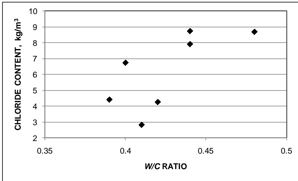
Figure 114. Graph. Average chloride content at a depth of 25 mm (1 inch) versus w/c ratio at end of field tests.
