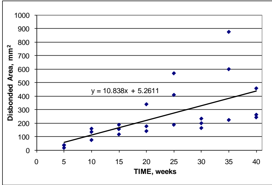
Figure 217. Graph. Rapid macrocell test, disbonded area versus time for specimens with ECR.
