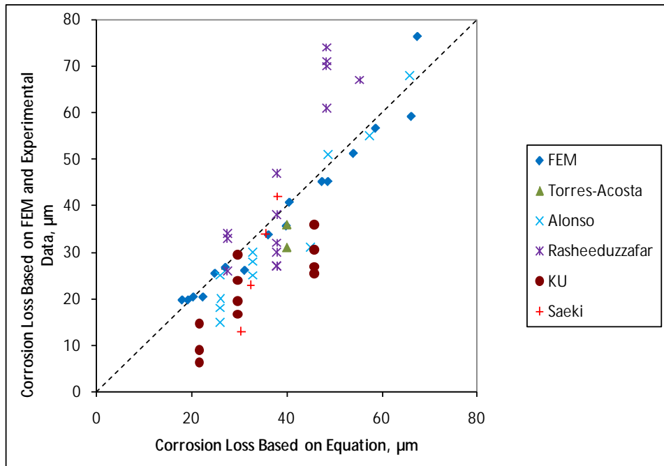
Figure 255. Graph. Corrosion loss to crack concrete for uniform general corrosion based on experimental and finite element results versus predicted corrosion losses using figure 252.
