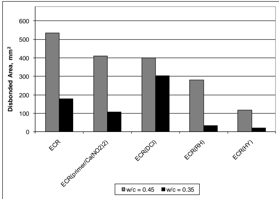
Figure 112. Graph. Comparison of disbondment of top bars in southern exposure specimens cast in concrete with w/c = 0.35 and 0.45.
