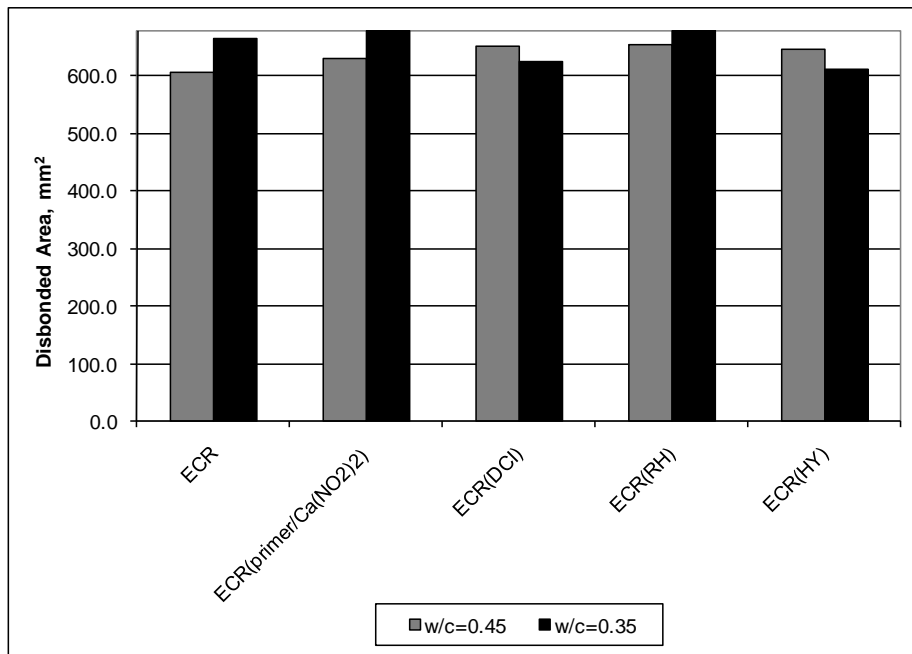
Figure 113. Graph. Comparison of disbondment of top bars in cracked beam specimens cast in concrete with w/c = 0.35 and 0.45.
