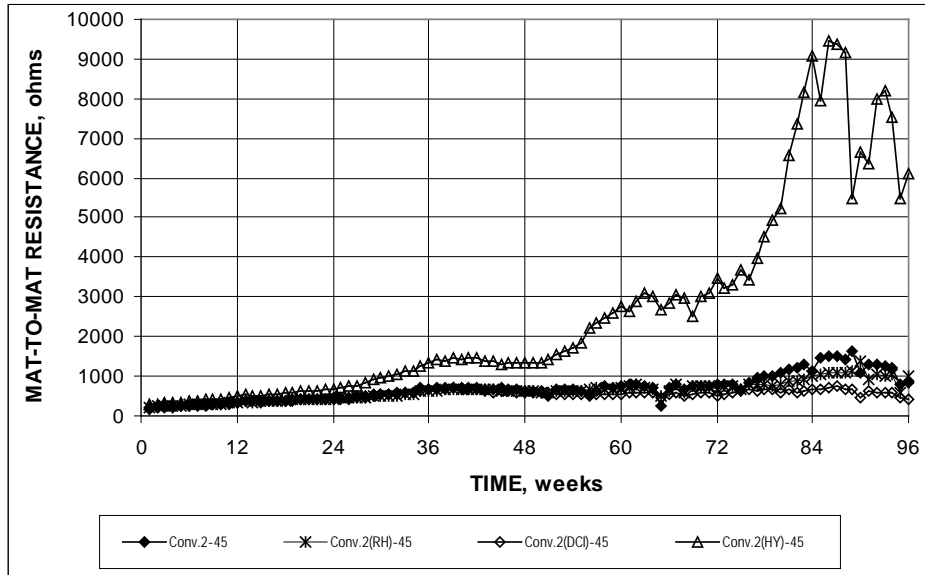
Figure 92. Graph. Cracked beam test, mat-to-mat resistance for conventional reinforcement in specimens containing corrosion inhibitors.
