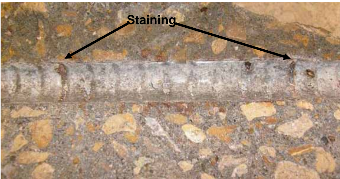
Figure 249. Photo. Concrete surrounding test bar from specimen ECR-2r-H-2.
