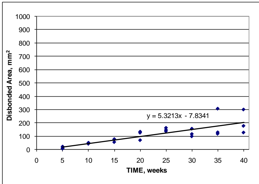
Figure 218. Graph. Rapid macrocell test, disbonded area versus time for specimens with MC reinforcement.
