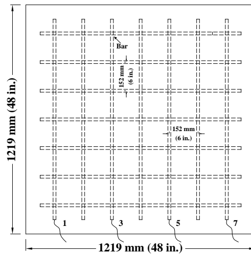
Figure 17. Illustration. Field test specimens, bottom slab.
