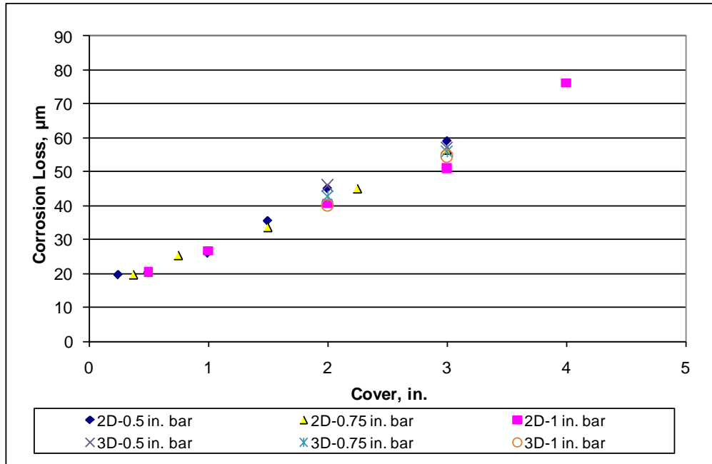
Figure 259. Graph. Corrosion loss to crack concrete for uniform general corrosion versus cover for two-and three-dimensional finite element model.
