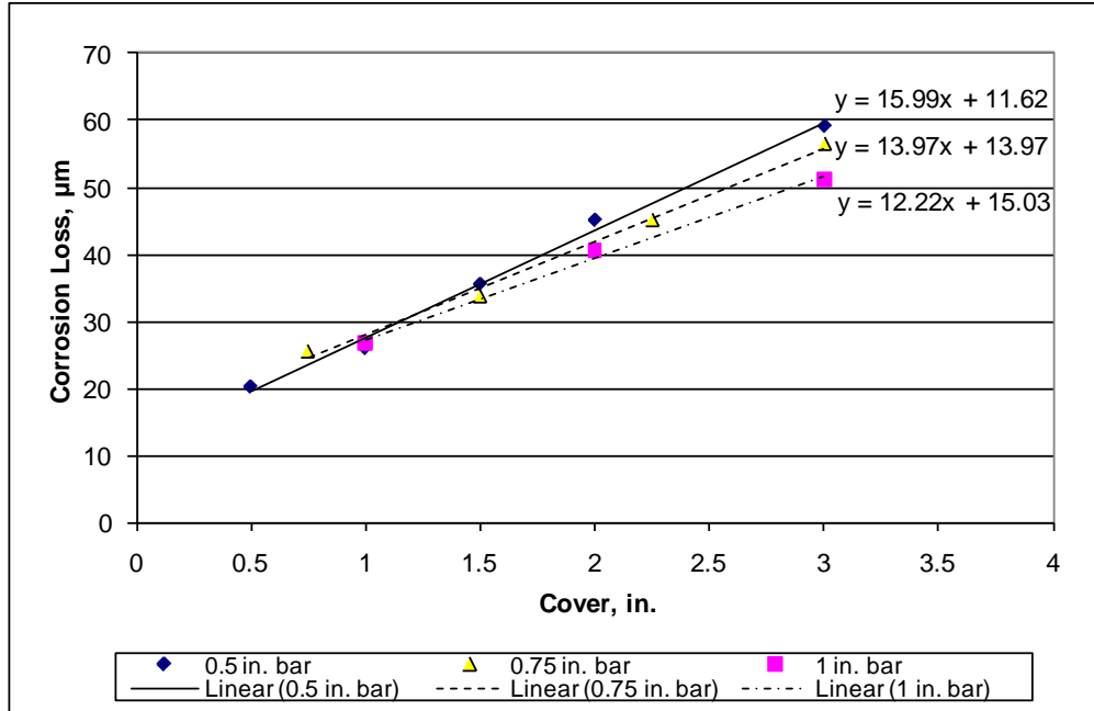
Figure 251. Graph. Corrosion loss to crack concrete versus cover showing effect of bar diameter for two-dimensional finite element model.
