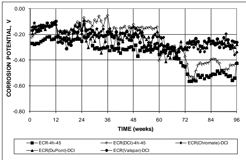
Figure 64. Graph. Southern exposure test, corrosion potential of top mat for conventional ECR with and without corrosion inhibitor and increased-adhesion ECR with corrosion inhibitor.
