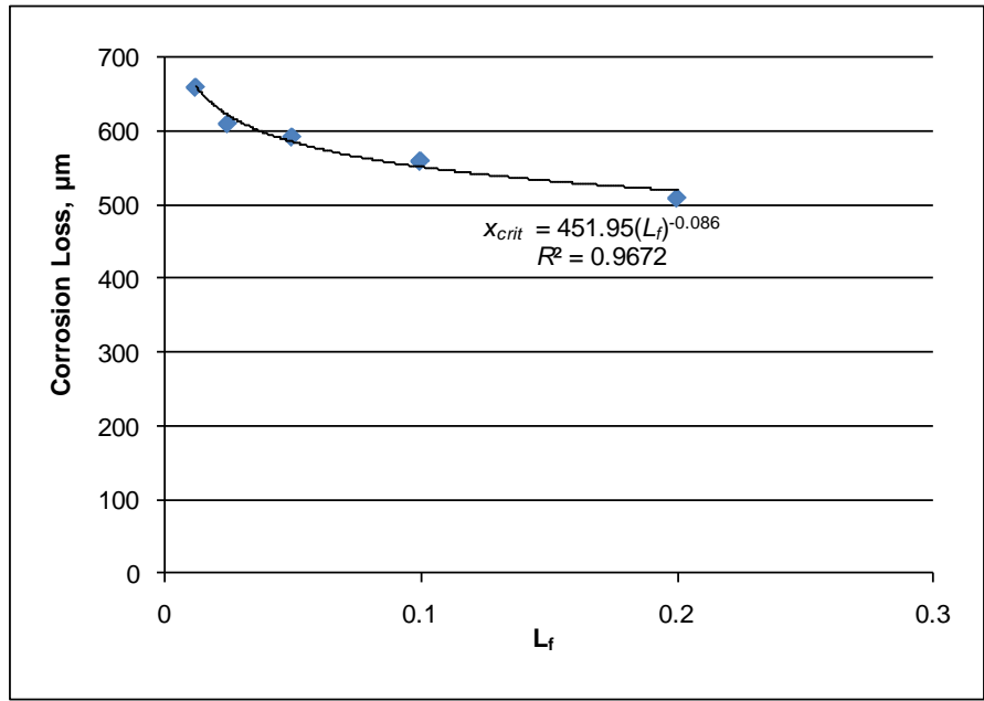
Figure 262. Graph. Corrosion loss to crack concrete x_{crit} versus L_f with best fit line for 1,013-mm 2 (1.57-in 2 ) corroding area.
