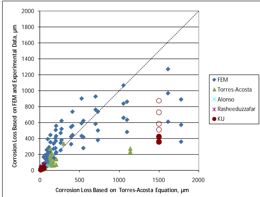
Figure 270. Graph. Corrosion loss in localized corrosion specimens versus corrosion loss predicted by the equation in figure 268 with three-dimensional finite element model and experimental data (revised scale).
