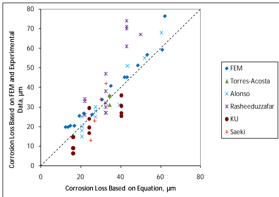
Figure 258. Graph. Corrosion loss to crack concrete for uniform general corrosion based on experimental and finite element results versus predicting corrosion losses using figure 256.
