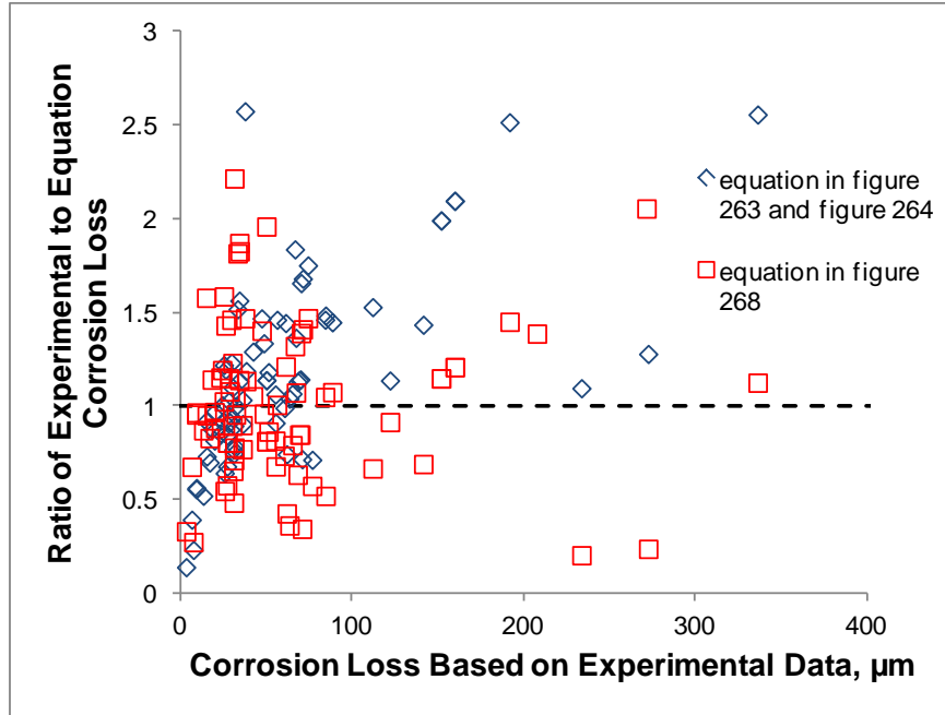
Figure 271. Graph. Ratio of experimentally derived corrosion loss to predicted corrosion loss versus corrosion loss to crack concrete based on experimental data.
