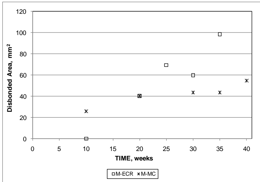
Figure 221. Graph. Disbonded area versus time for ECR and MC reinforcement in simulated pore solution without salt.
