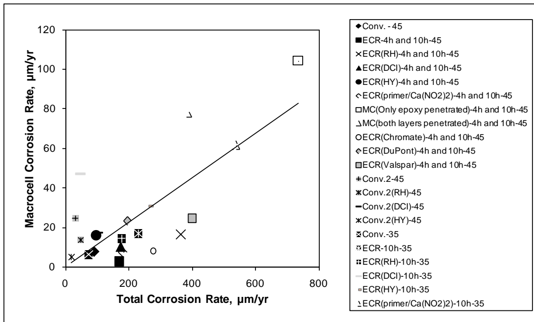
Figure 100. Graph. Cracked beam specimens, average total and macrocell corrosion rates based on losses after corrosion initiation based on total area for conventional reinforcement and area exposed at holes through coating for coated reinforcement, w/c = 0.45 or 0.35.
