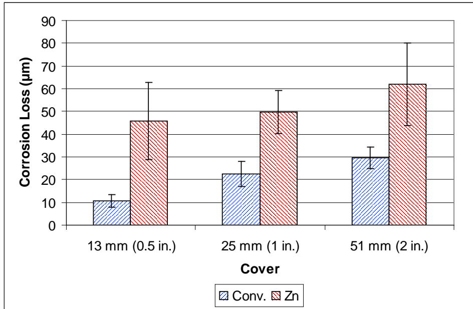
Figure 232. Graph. Average corrosion loss required to crack concrete for specimens with conventional and galvanized reinforcement.
