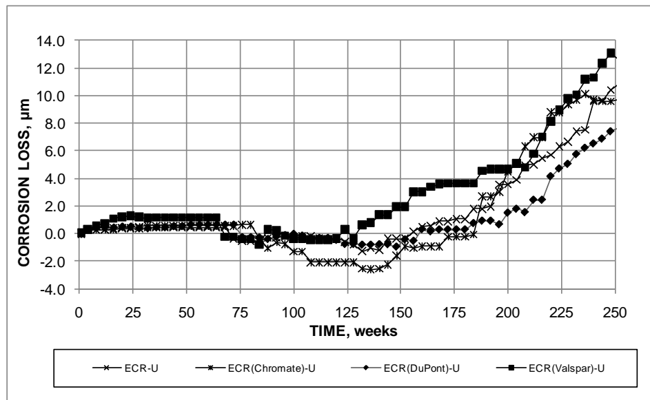
Figure 121. Graph. Field test, average corrosion losses based on area exposed at holes through coating for conventional and increased-adhesion ECR without simulated cracks.
