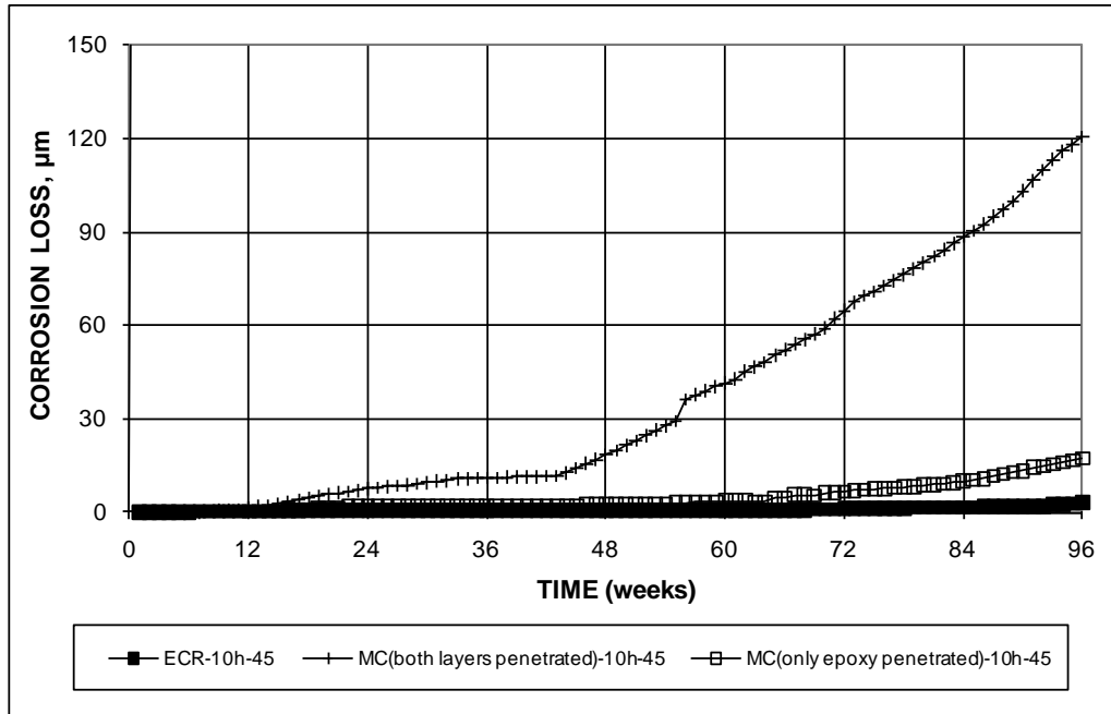
Figure 66. Graph. Southern exposure test, corrosion loss based on area exposed at holes through coating for conventional ECR and MC reinforcement with bars containing 10 holes.
