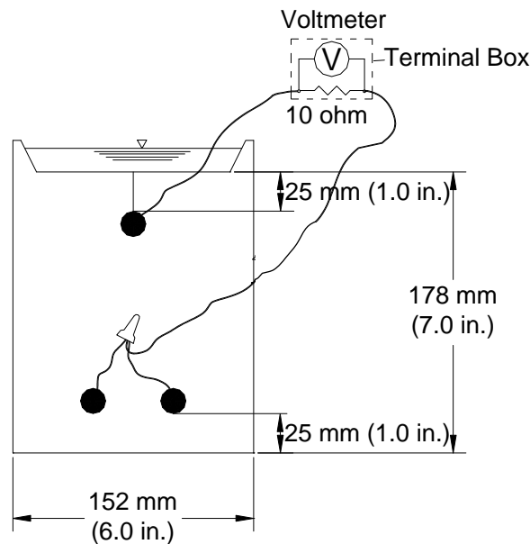
Figure 11. Illustration. Cracked beam test specimen.
