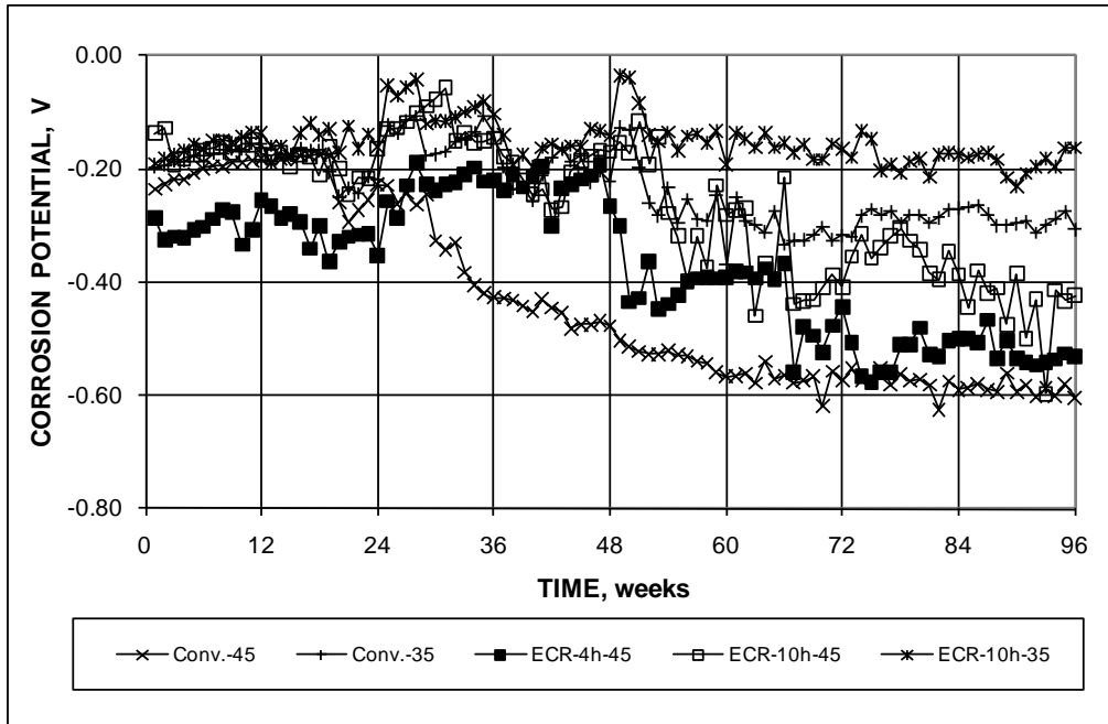
Figure 52. Graph. Southern exposure test, corrosion potential of bottom mat for conventional reinforcement and ECR.
