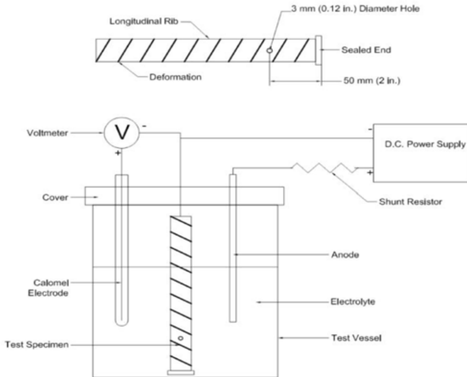
Figure 1. Illustration. Cathodic disbondment test setup (after reference 13).
