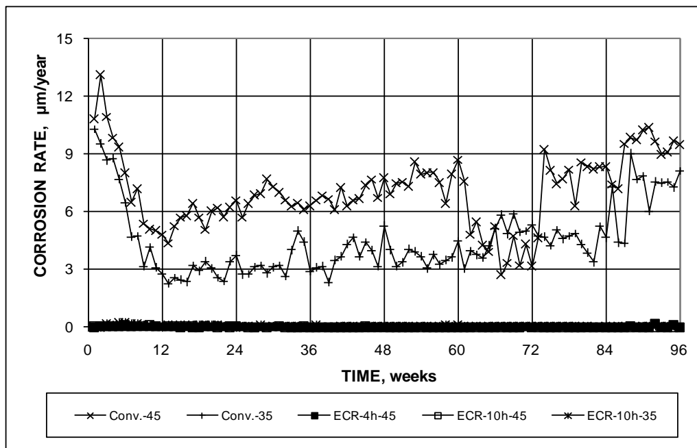
Figure 75. Graph. Cracked beam test, average corrosion rates based on total area of control specimens for conventional reinforcement and ECR.
