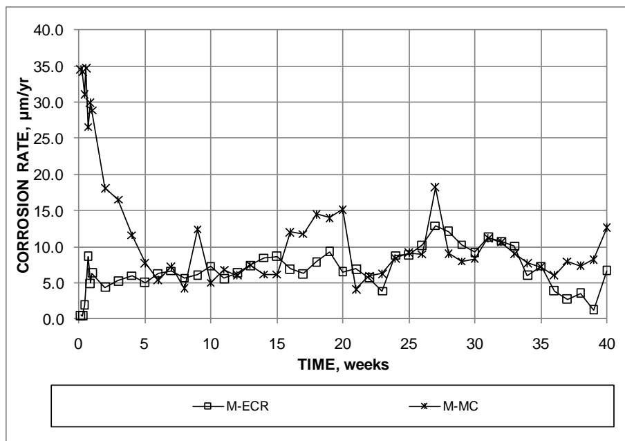
Figure 204. Graph. Rapid macrocell test, average corrosion rate based on total area of ECR and MC reinforcement.
