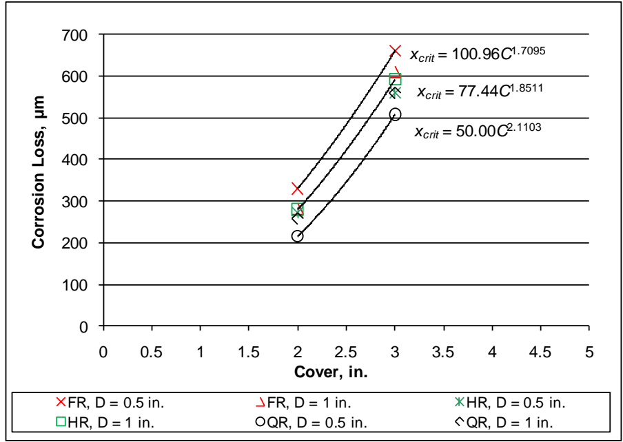
Figure 261. Graph. Corrosion loss to crack concrete x_{crit} versus cover C for 1,013-mm 2 (1.57-in 2 ) corroding area.
