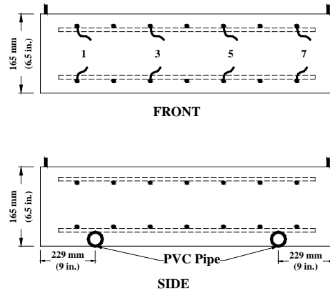
Figure 18. Illustration. Field test specimens, front and side views.
