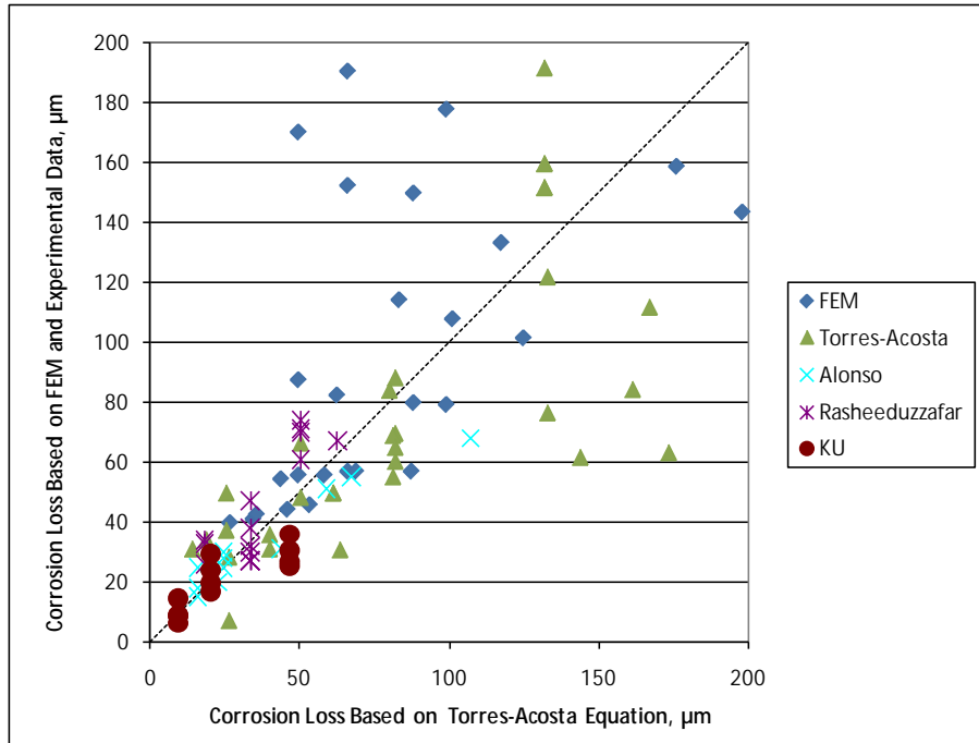
Figure 269. Graph. Corrosion loss in localized corrosion specimens versus corrosion loss predicted by the equation in figure 268 with three-dimensional finite element model and experimental data.
