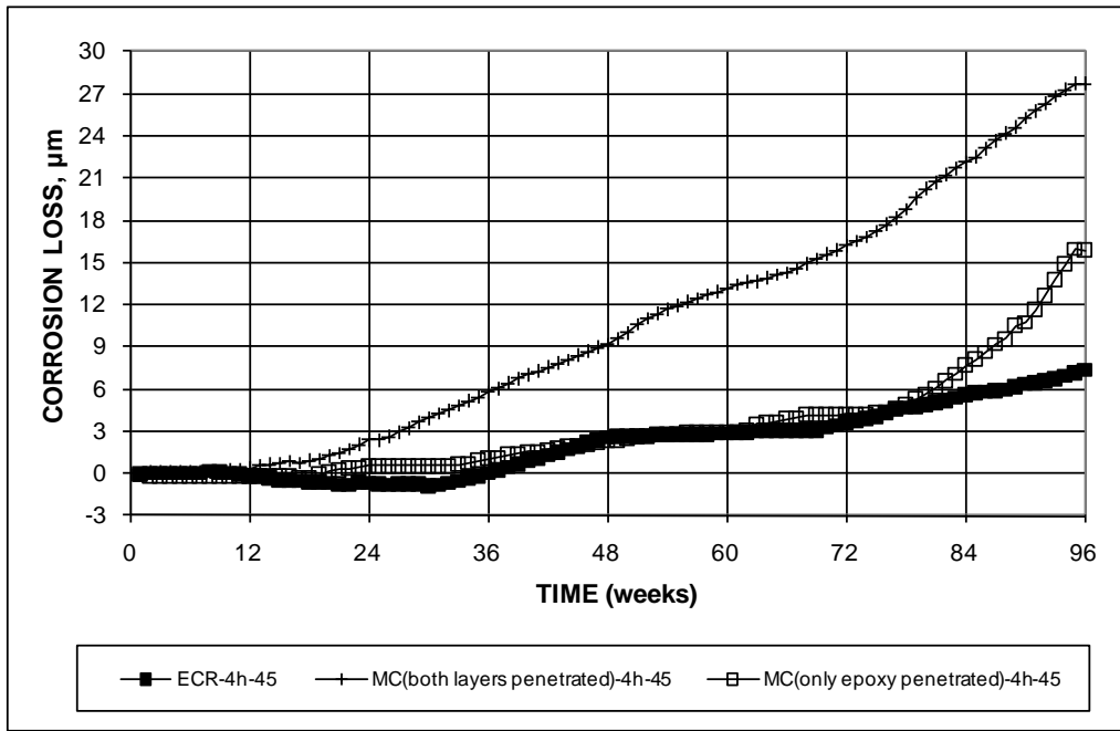
Figure 65. Graph. Southern exposure test, corrosion loss based on area exposed at holes through coating for conventional ECR and MC reinforcement with bars containing four holes.
