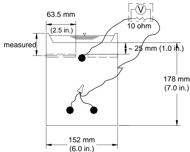
Figure 12. Illustration. Corrosion initiation beam test specimen.
