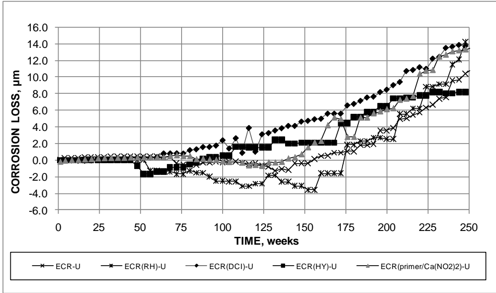
Figure 127. Graph. Field test, average corrosion losses based on area exposed at holes through coating for conventional ECR without and with corrosion inhibitors and without simulated cracks.
