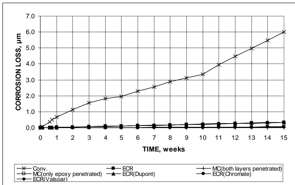
Figure 32. Graph. Macrocell test, average corrosion loss based on total area for bare conventional, ECR, increased-adhesion ECR, and MC steel in simulated pore solution with 1.6 molal ion concentration of sodium chloride.
