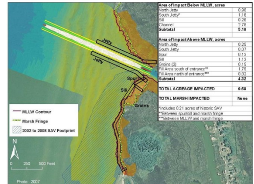
Figure 2. Jetty design for Rhodes Point entrance channel, MD
