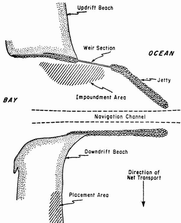
Figure 4. Weir jetty with impoundment area between jetties.
