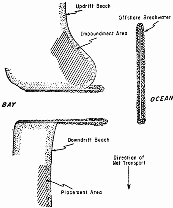
Figure 3. Impoundment area behind detached offshore breakwater.
