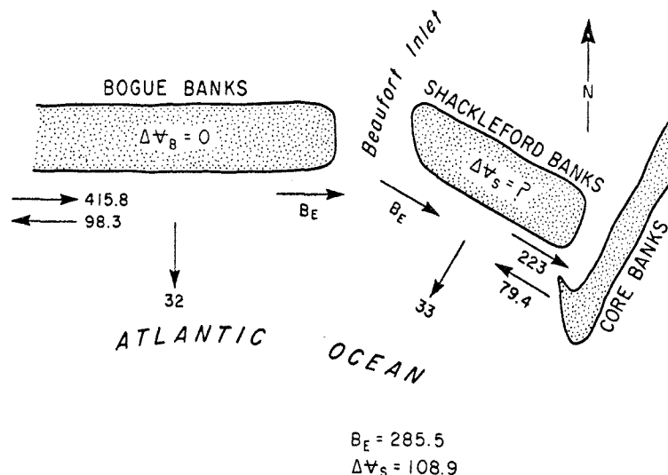
Figure 28. Weir-jetty construction sediment budget for strategy 4.
