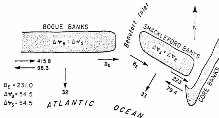
Figure 27. Weir-jetty construction sediment budget for strategy 3.
