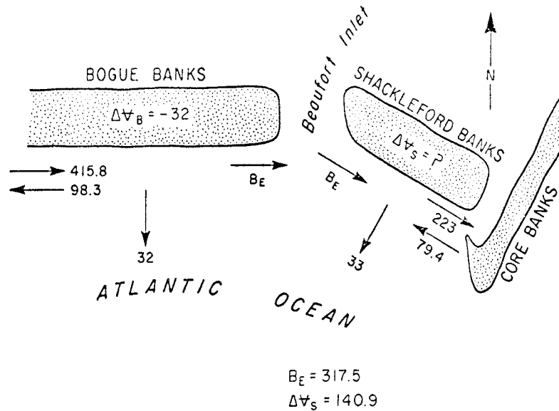
Figure 25. Weir-jetty construction sediment budget for strategy 1.
