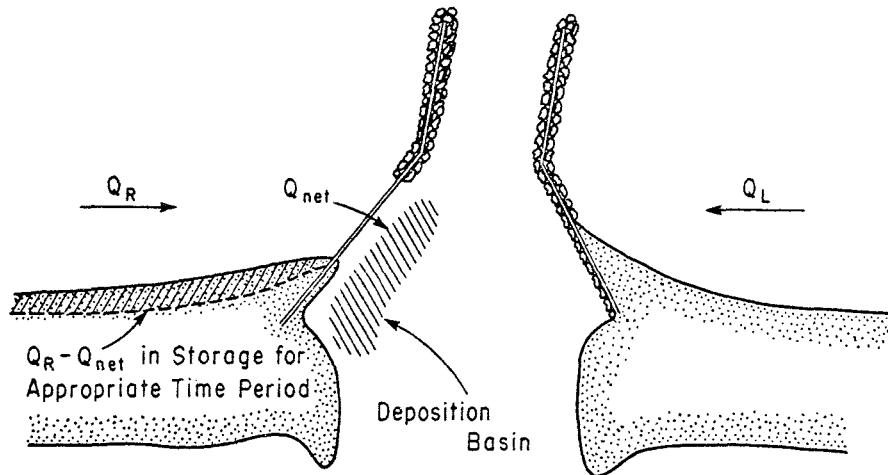
Figure 7. Sand transport and storage at an ideal weir-jetty system.
