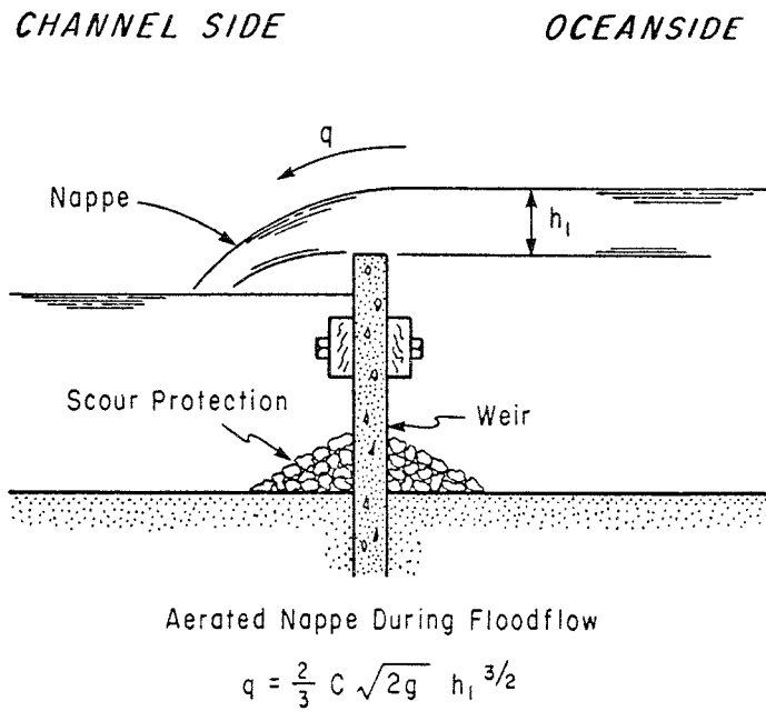
Figure 12. Definition sketch of flow across weir with aerated nappe.
