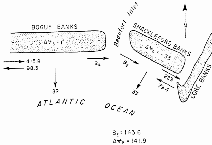
Figure 26. Weir-jetty construction sediment budget for strategy 2.
