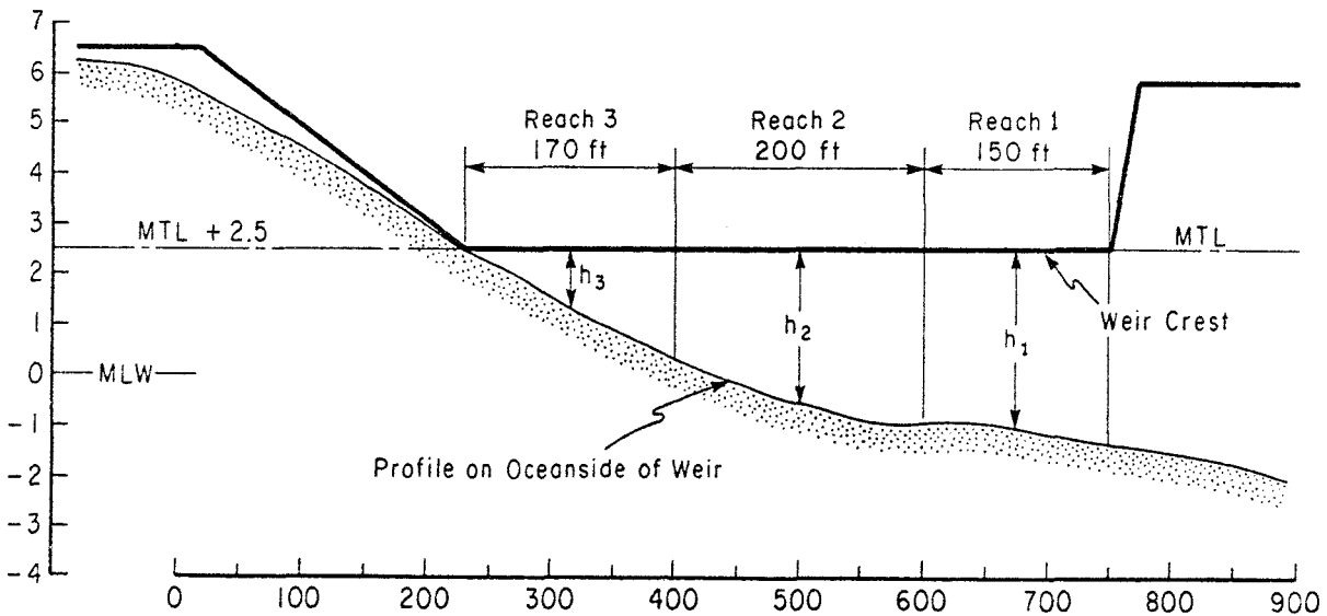
Figure 17. Beach profile adjacent to weir section.
