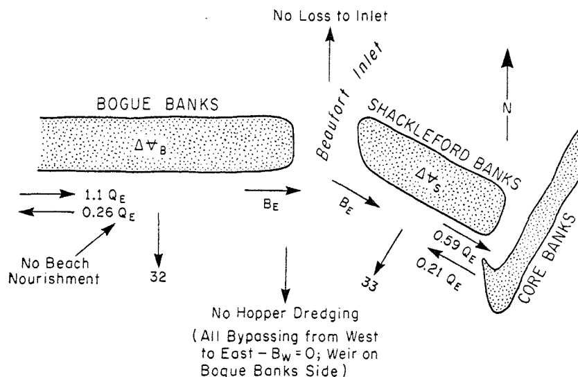
Figure 24. Typical sediment budget conditions after weir-jetty construction.
