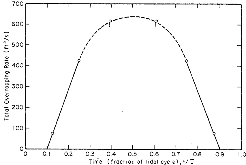
Figure 18. Time variation of overtopping rate.
