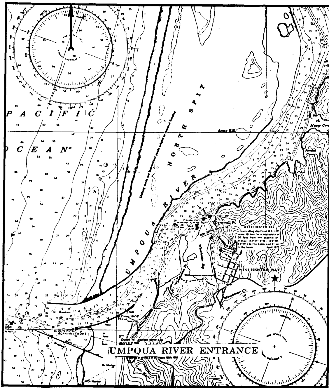
Figure 14. Umpqua River, Oregon, in 1970 (from National Ocean Survey chart 6004).
