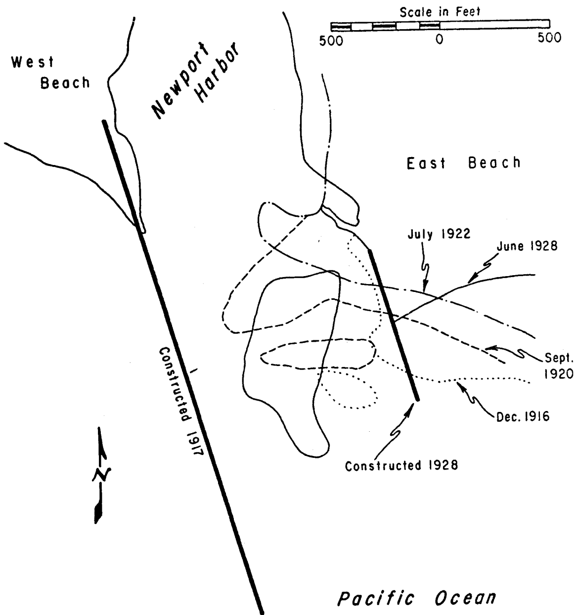
Figure 29. Entrance to Newport Harbor, California (after a 1928 map by the Newport city engineer).
