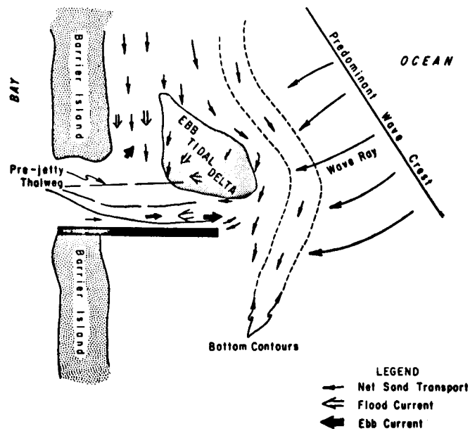
Figure 32. Idealized model of channel migration and shoreline response subsequent to construction of a single downdrift jetty.
