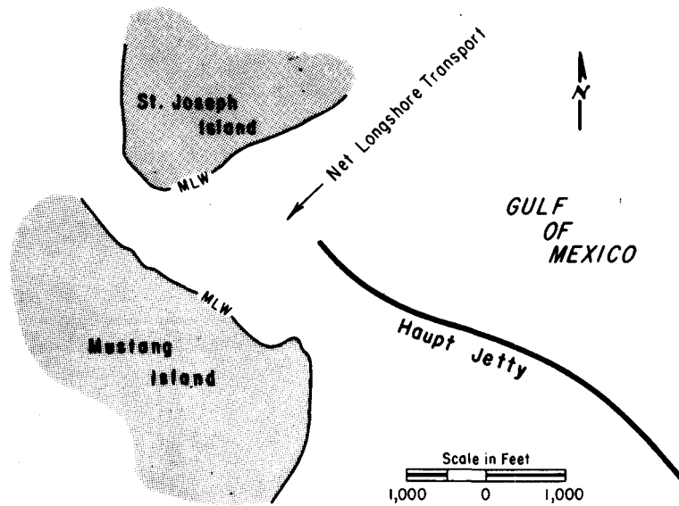
Figure 2. Aransas Pass, Texas (after U.S. Army, Corps of Engineers, 1908).
