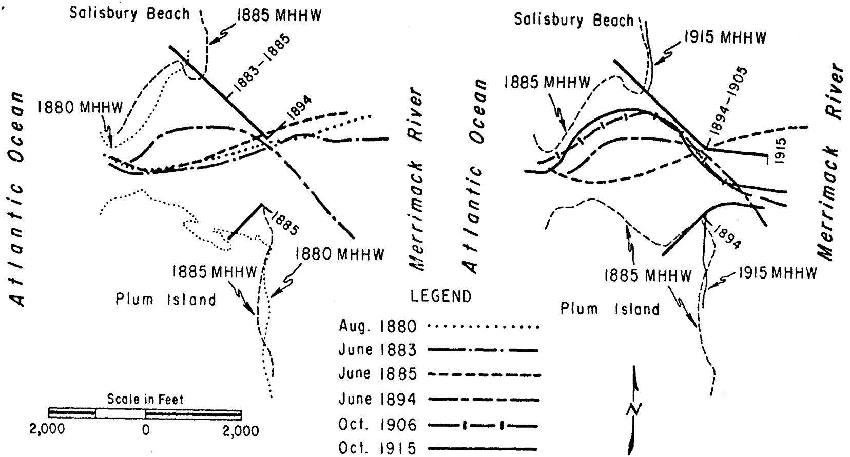
Figure 28. Time history of channel thalwegs, Merrimack River, Massachusetts, August 1880-October 1915 (after U.S. Army Engineer Division, New England, surveys).
