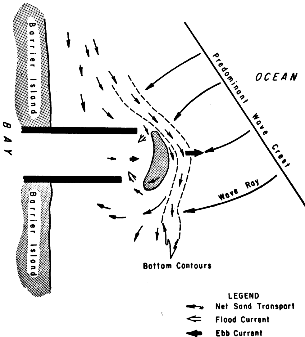
Figure 5. Current pattern at a twin-jettied inlet.
