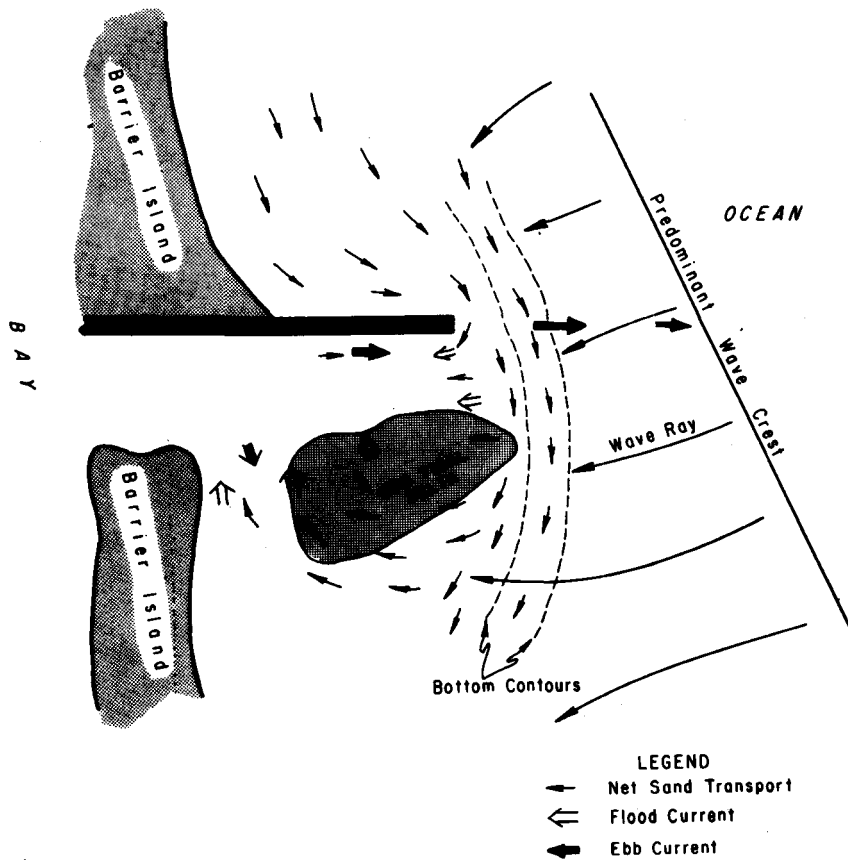
Figure 3. Current pattern at a single updrift jetty.
