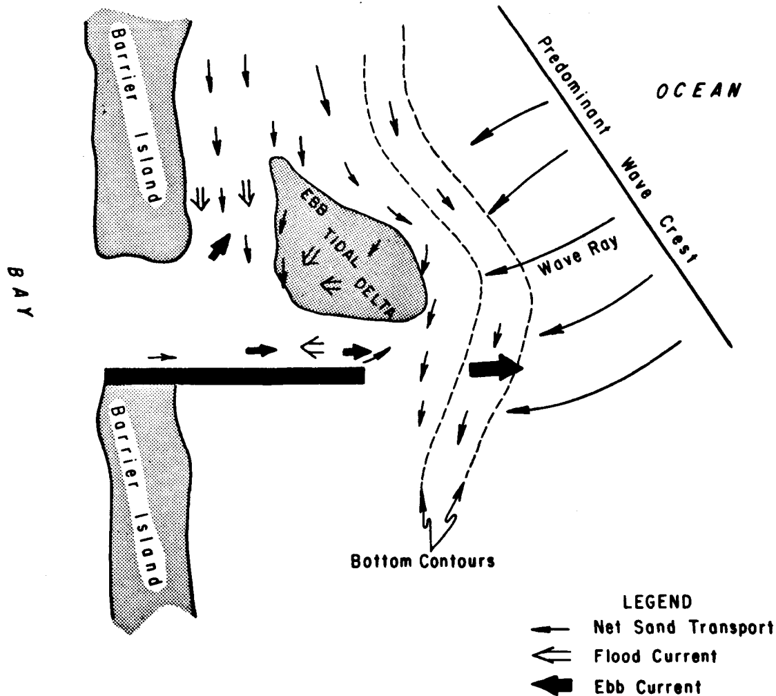
Figure 4. Current pattern at a single downdrift jetty.
