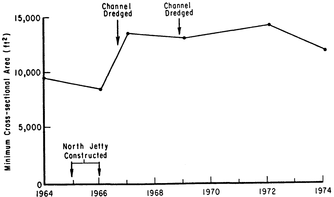
Figure 18. Time history of minimum channel area below MSL, Masonboro Inlet, North Carolina.
