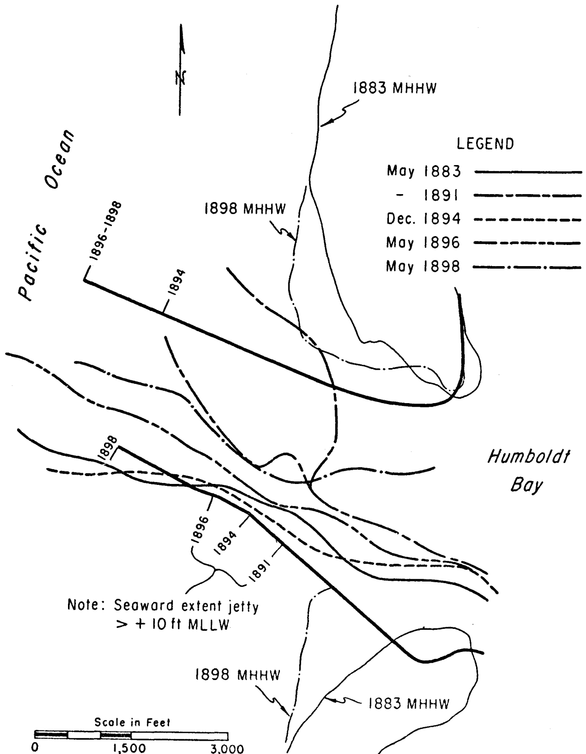
Figure 21. Time history of channel thalwegs, Humboldt Bay, California, May 1883-May 1898 (after U.S. Army Engineer District, San Francisco, surveys).
