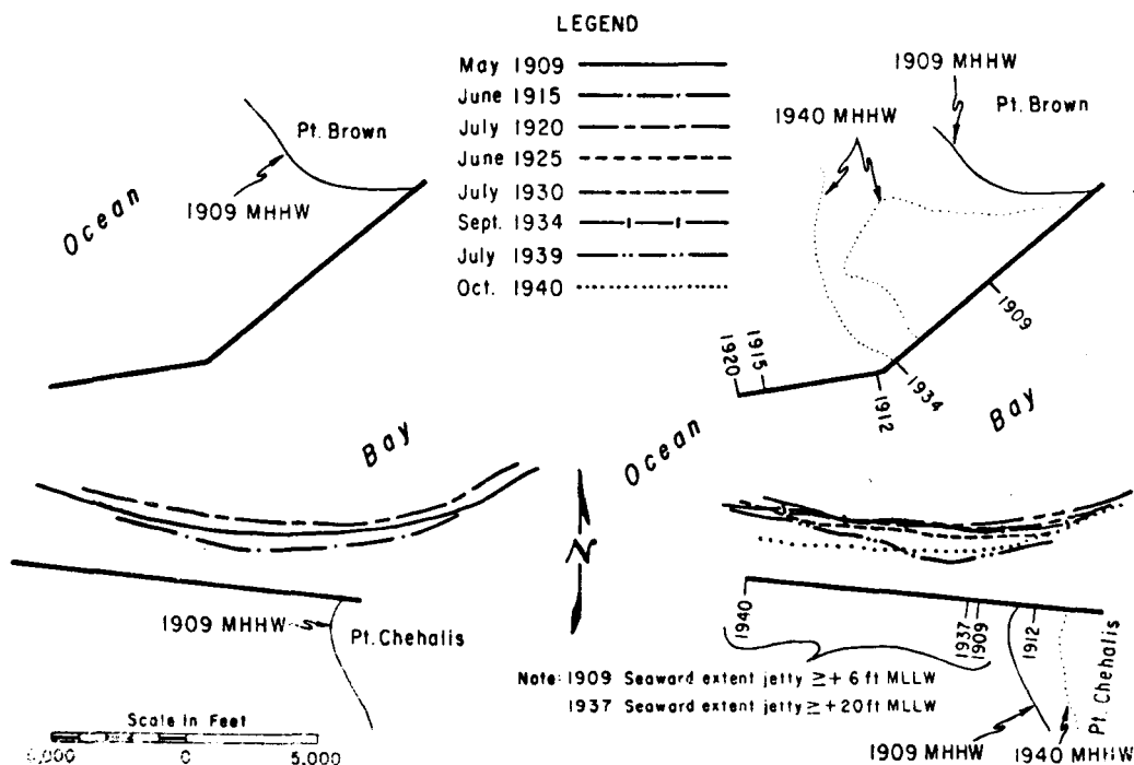
Figure 8. Time history of channel thalwegs, Grays Harbor, Washington, May 1909–October 1940 (after U.S. Army Engineer District, Seattle, surveys).
