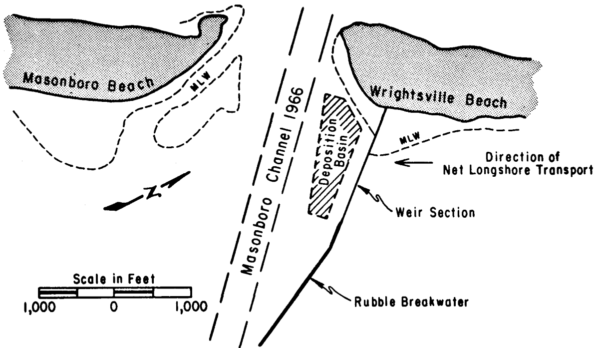
Figure 1. Masonboro Inlet, North Carolina (after U.S. Army, Corps of Engineers, Coastal Engineering Research Center, 1977).
