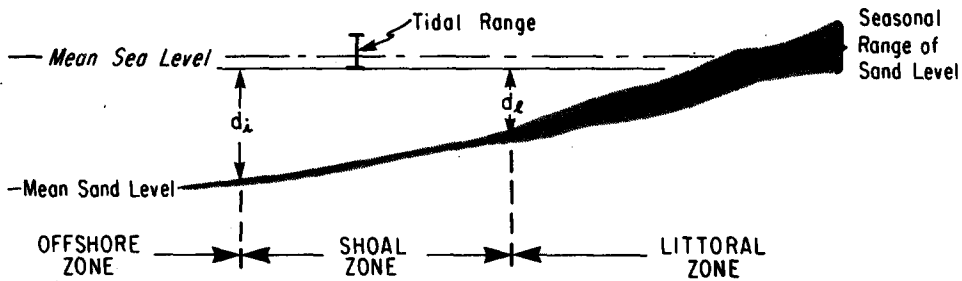
Fig. 1. Proposed annual zonation of seasonal sand beach profile; d_i is maximum water depth for motion initiation by median wave condition, and d_e is maximum water depth for nearshore erosion by extreme (12 hours per year) wave condition.
