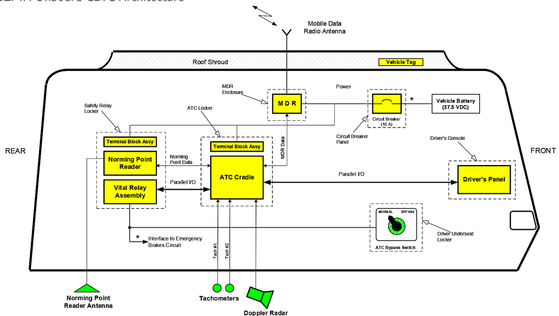
Figure 5-3 SEPTA Onboard CBTC Architecture
