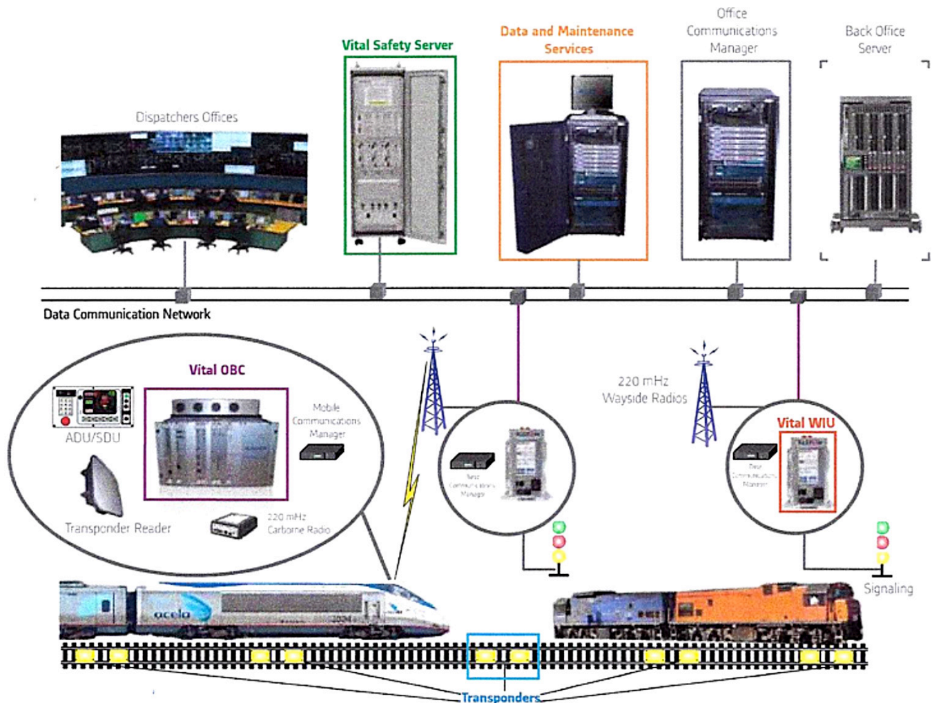
ACSES System Diagram
