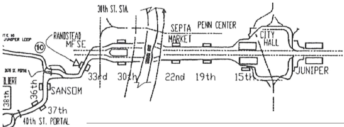
SEPTA Light Rail Tunnel Track Plan
