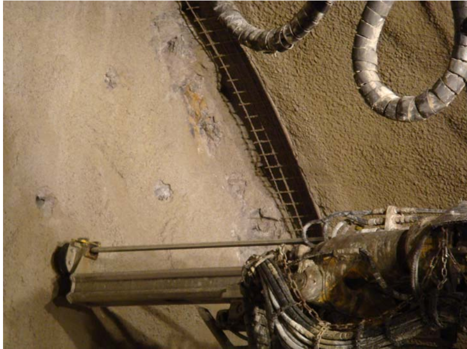
Figure 9-11 Shotcrete Lining Installed at the Face in a SEM Tunnel Excavated by Drill-and-Blast (Andrea Tunnel, Austria)
