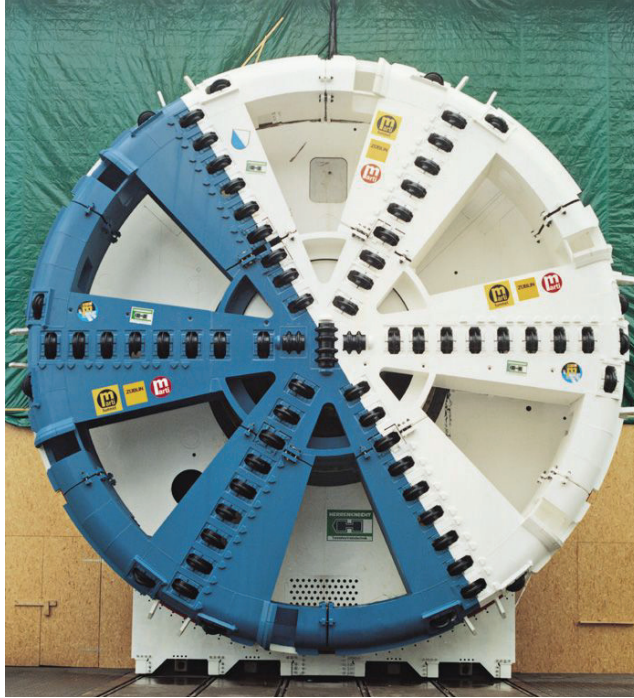
Figure D-6 above shows the cutterhead of the Herrenknecht S-256 Single Shield TBM used in the construction of the Isisberg tunnel, Switzerland, which on completion will be the longest underground section of the western Zurich bypass, will be directing transit traffic to central Switzerland around the city. The diameter of the cutterhead is about 38' (11.8 m). See Table D-1 for more data about the machine (Herrenknecht).
