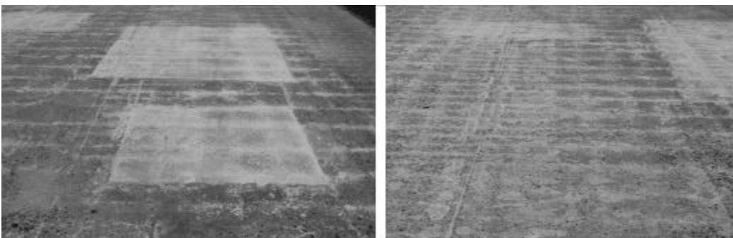
Figure 24. Layer of white material formed on the concrete surface directly above the reinforcing steel following ECE on an actual bridge deck [70]
