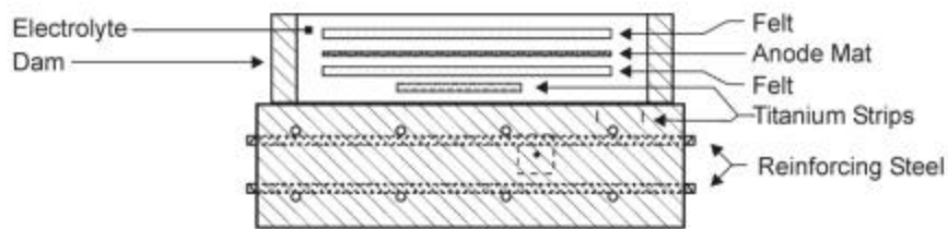
Section A-A: Side View Illustrating ECE Measurement Points (Not to Scale)
