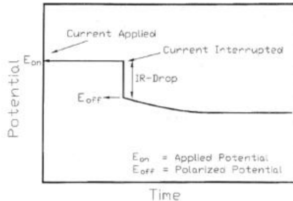
Figure 7. Change in voltage after interruption of applied current [66]
