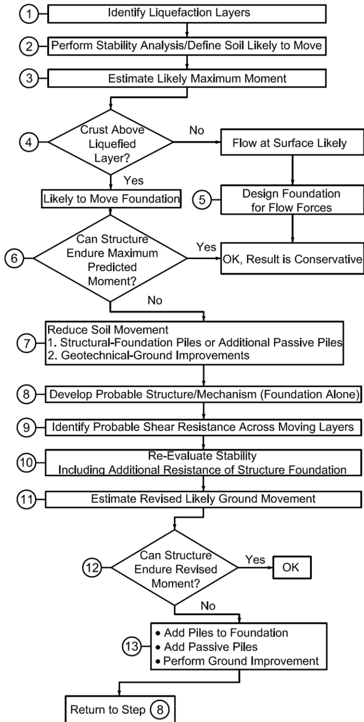
Figure 7-35 Design Flowchart
