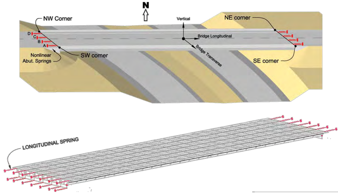
Figure 12-17 Bridge and Abutment Model
