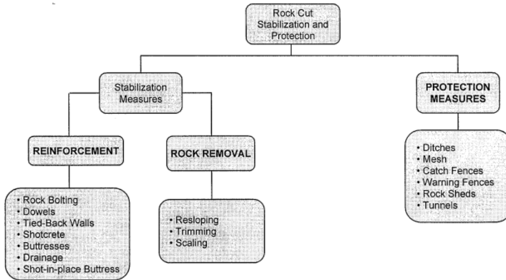
Figure 7-27 Categories of Rock Slope Stabilization Measures (FHWA 1998a)
