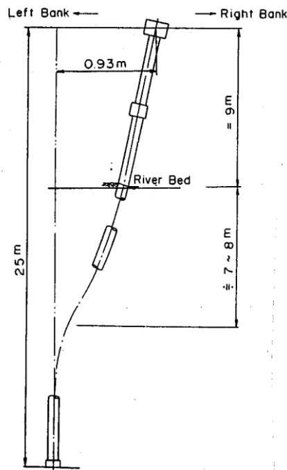
Figure 7-16 Deformation of a Steel Pipe pile for the Showa Bridge (Hamada, 1992)
