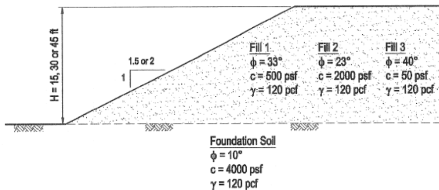
Figure 7-21 Slope Geometry
