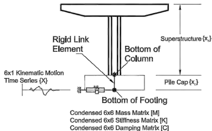
Figure 9-9 Implementation of Foundation Submodel in the Global Structural Model
