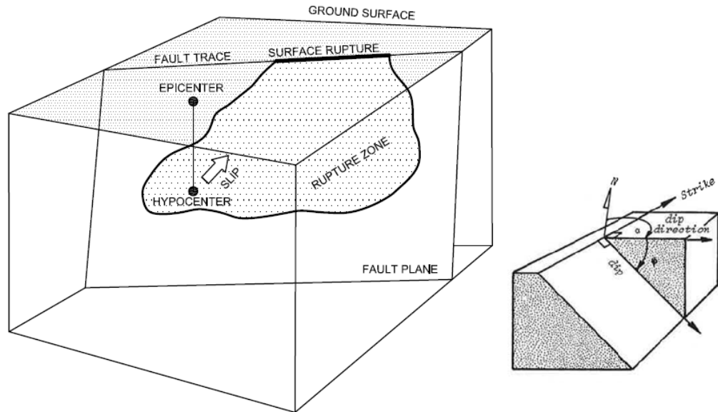
Figure 2-10 Basic Fault Geometry and Definition (after FHWA, 1998)
