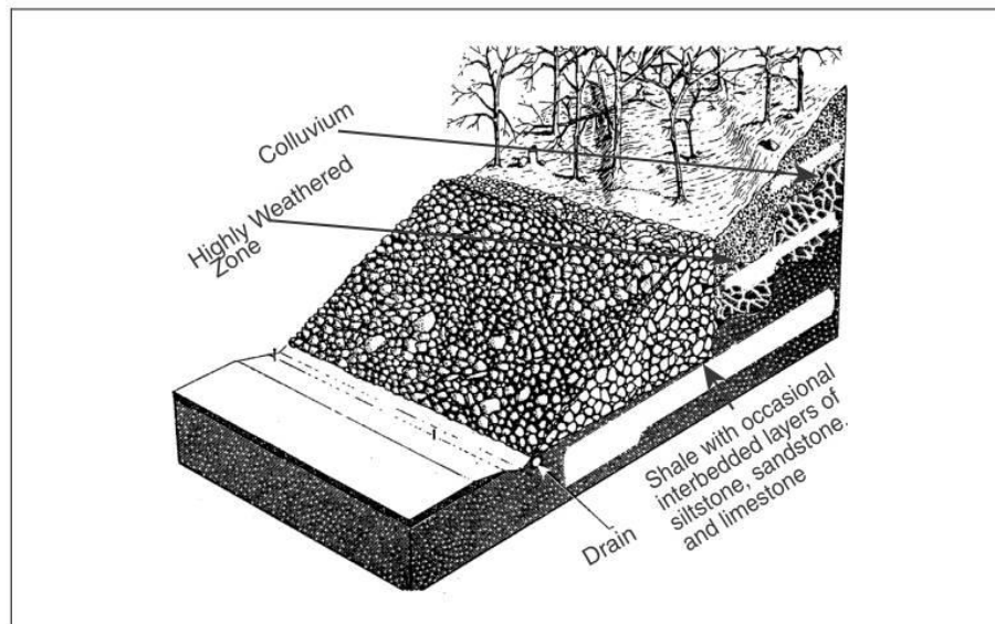
Figure 7-23 Rock Buttress Used to Increase Forces Resisting Slope Failure
