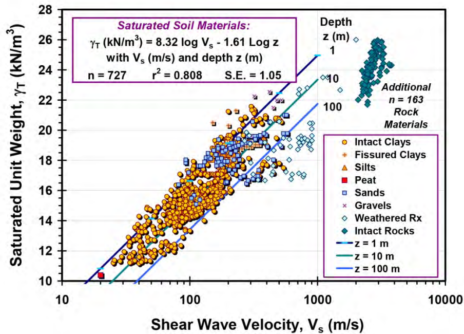
Figure 4-8 Correlation among Saturated Weight, Shear Wave Velocity, and Depth (Mayne, 2007)
