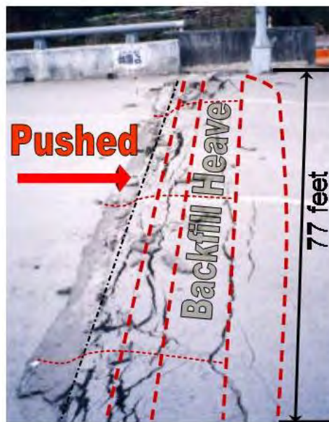
Figure 12-6 Formations of Mobilized Passive Wedges (Kosa et al., 2001)
