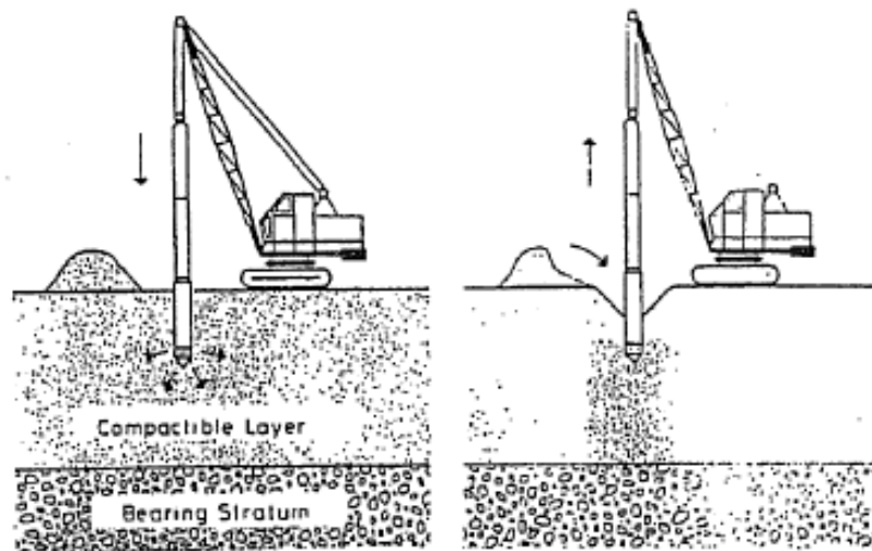
Figure 7-41 The Vibro Compaction Process
