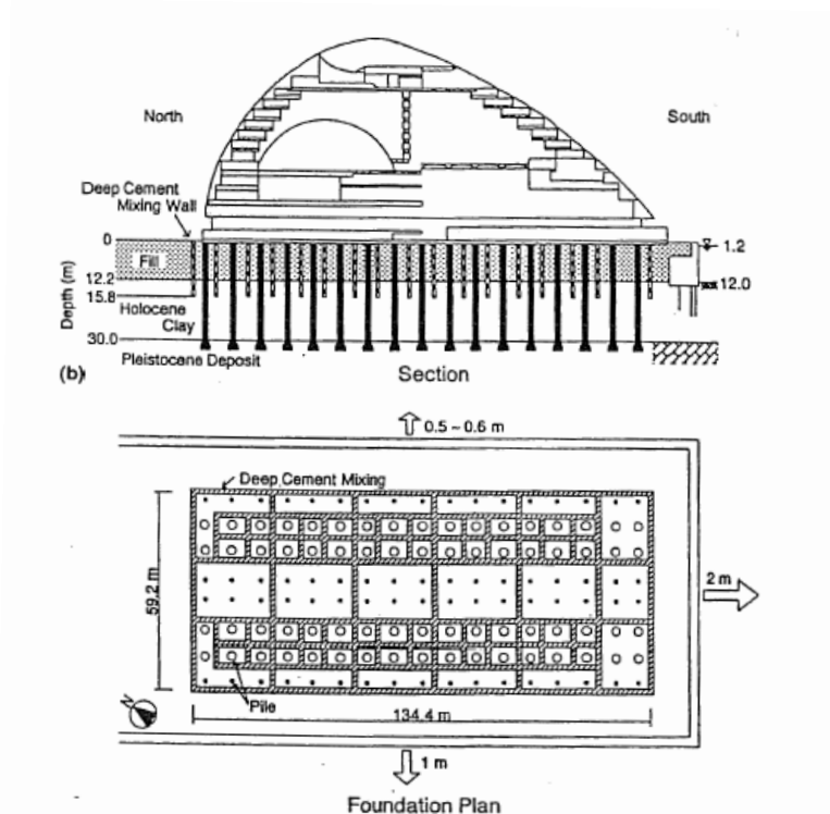
Figure 7-49 Kobe Hotel Foundation Plan
