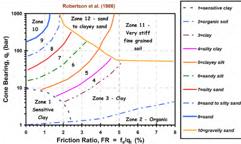
Figure 4-5 Soil Classification Chart Based on the CPT (Robertson et al., 1986)
