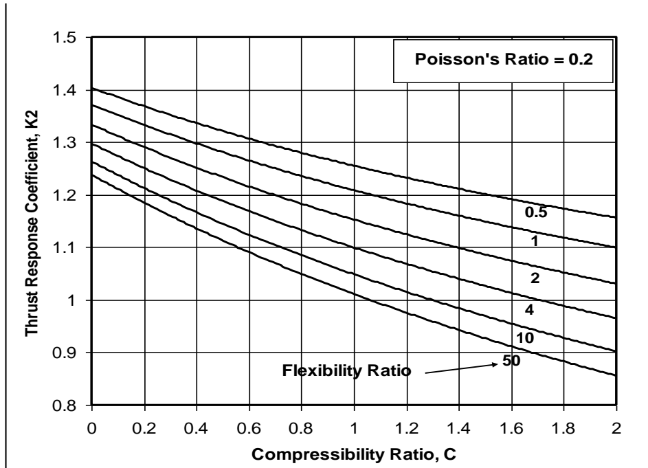
Figure 13-5 Lining Response Coefficient, K_2 , for Poisson's Ratio = 0.2 (No-Slip Interface Condition)
