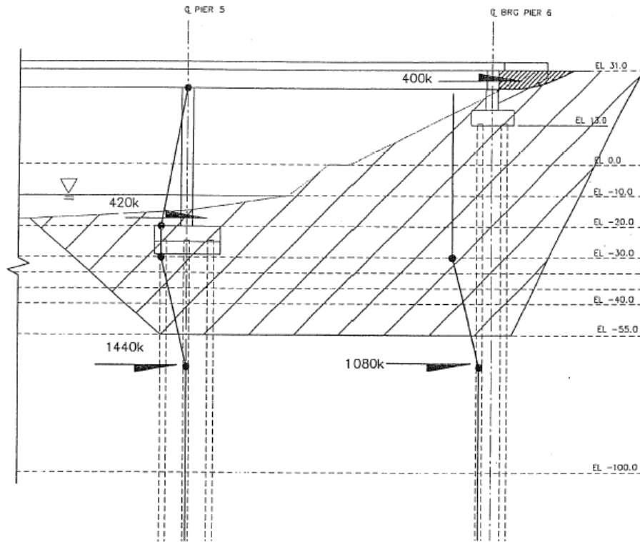
Figure 7-39 Forces Provided by Bridge and Foundation Piles for Resisting Lateral Spread
