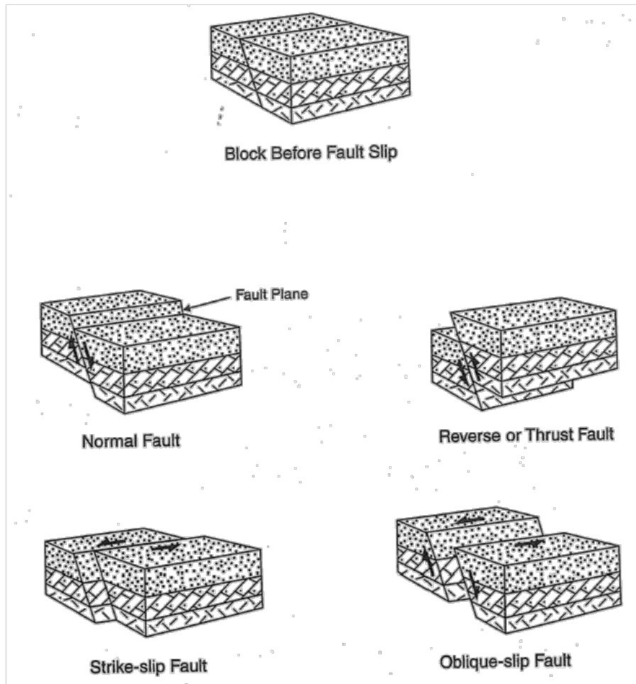
Figure 6-25 Types of Earthquake Faults
