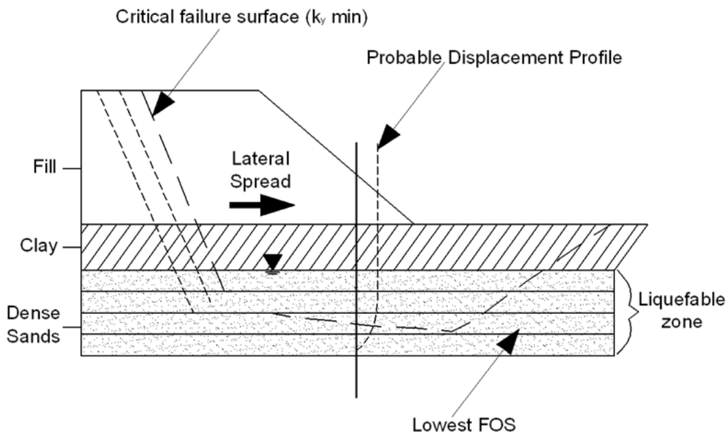
Figure 7-34 Pseudo-static Stability Analysis
