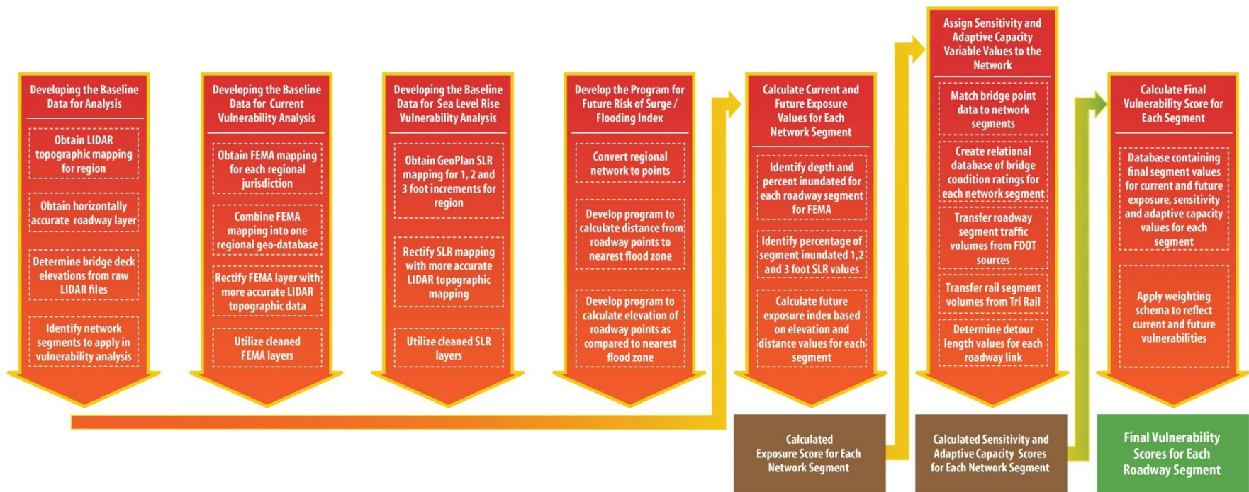
Figure 4: Technical Flow Diagram for Vulnerability Assessment
