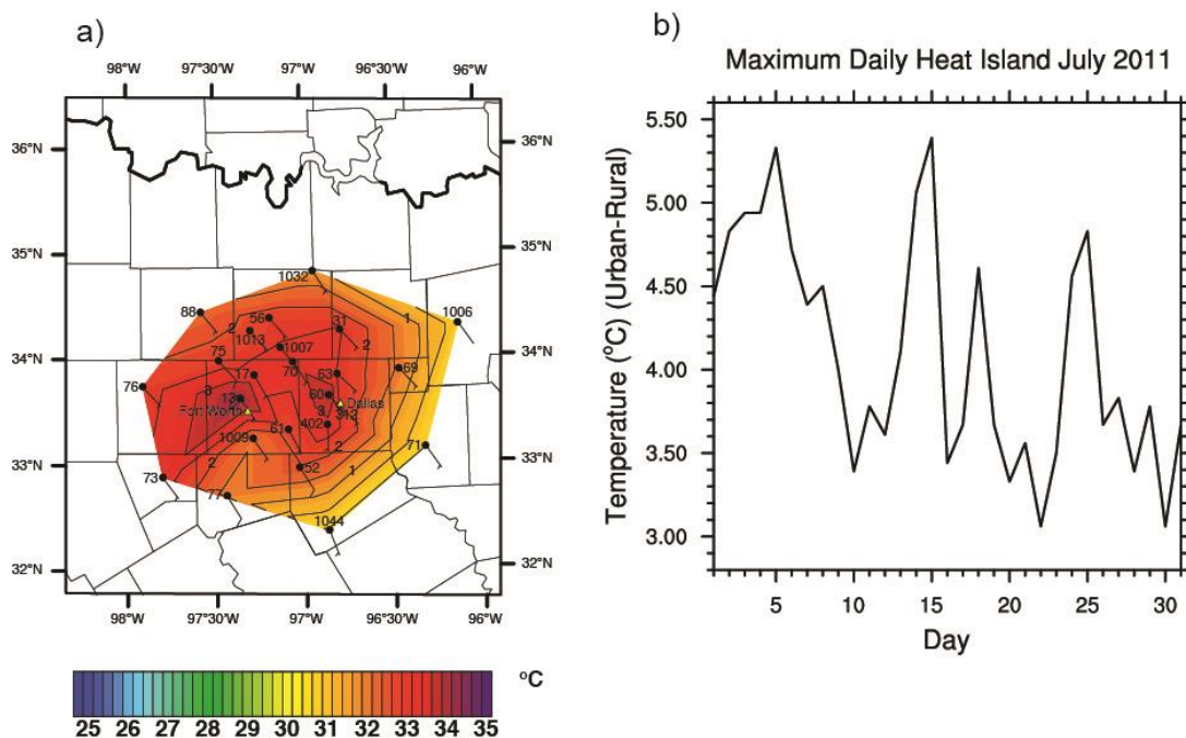
Figure 2.8. Maps of the average air temperatures ( ^{\circ}\text{C} ) at screen level at (a) 21:00, reported by TCEQ stations listed in Table II in Winguth et al. (2013). Wind barbs are in knots. Each short barb represents 5 knots and each long barb 10 knots. Contour lines show the magnitude of the urban heat island relative to the Kaufman station (CAMS 71). Contour line interval is 0.5^{\circ}\text{C} . b) Daily maximum urban heat island in July 2011.
