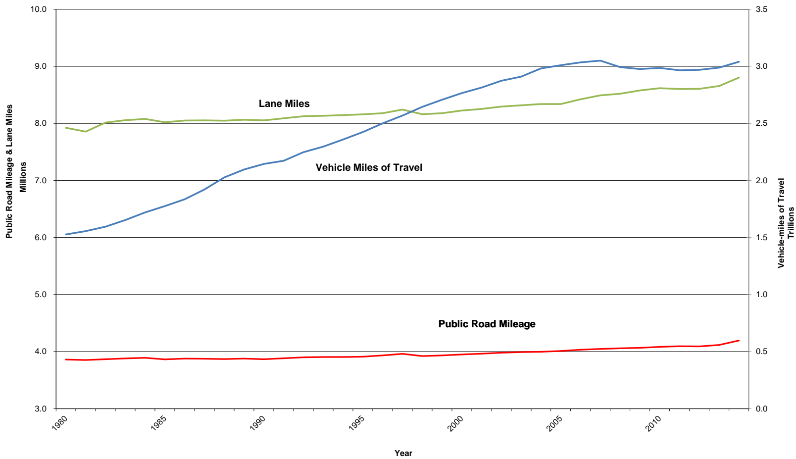
Public Road Mileage, Lane-Miles, and VMT 1980 - 2014
