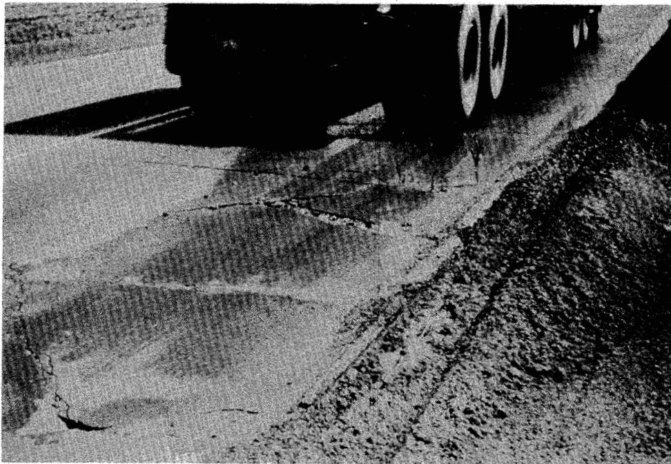
Figure 47. Pumping of concrete pavement.
