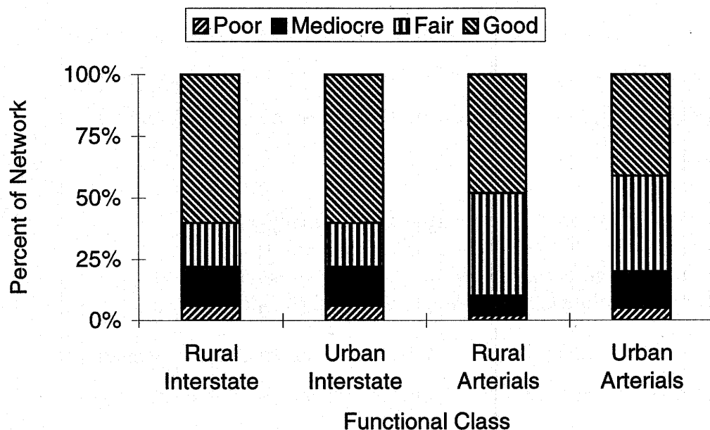
Figure 3. Distribution of pavement condition based on functional classification.
