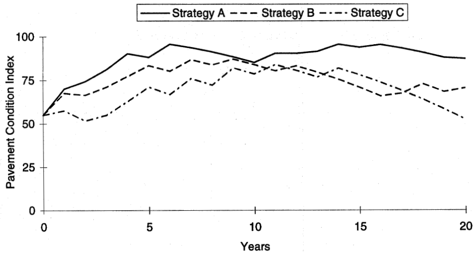
Figure 10. Average pavement condition for preventive maintenance, rehabilitation, and reconstruction.
