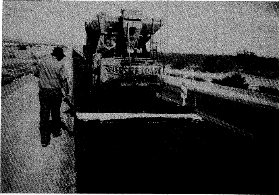
Figure 24. Applying slurry seal using a slurry machine.
