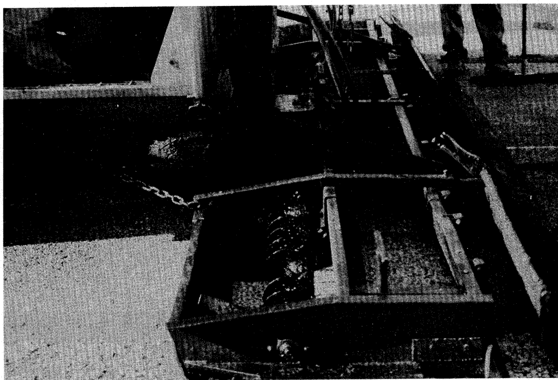
Figure 29. Spreader box of the micro-surfacing machine.
