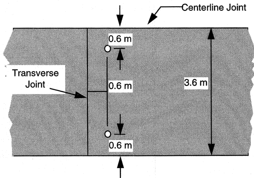
Figure 49. Typical hole pattern for jointed concrete pavements. (46)
