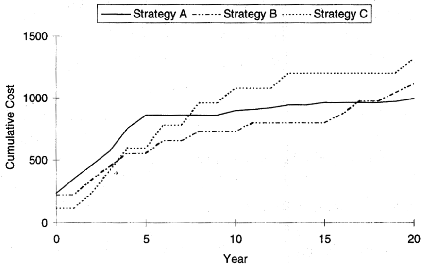
Figure 12. Comparison of different pavement preservation strategies.
