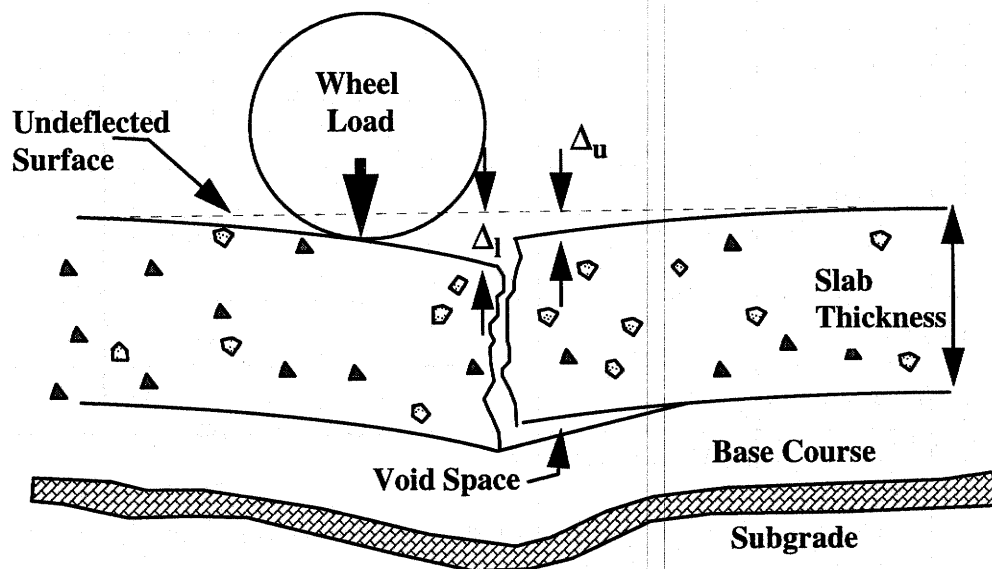
Figure 48. Concept of joint load transfer efficiency.
