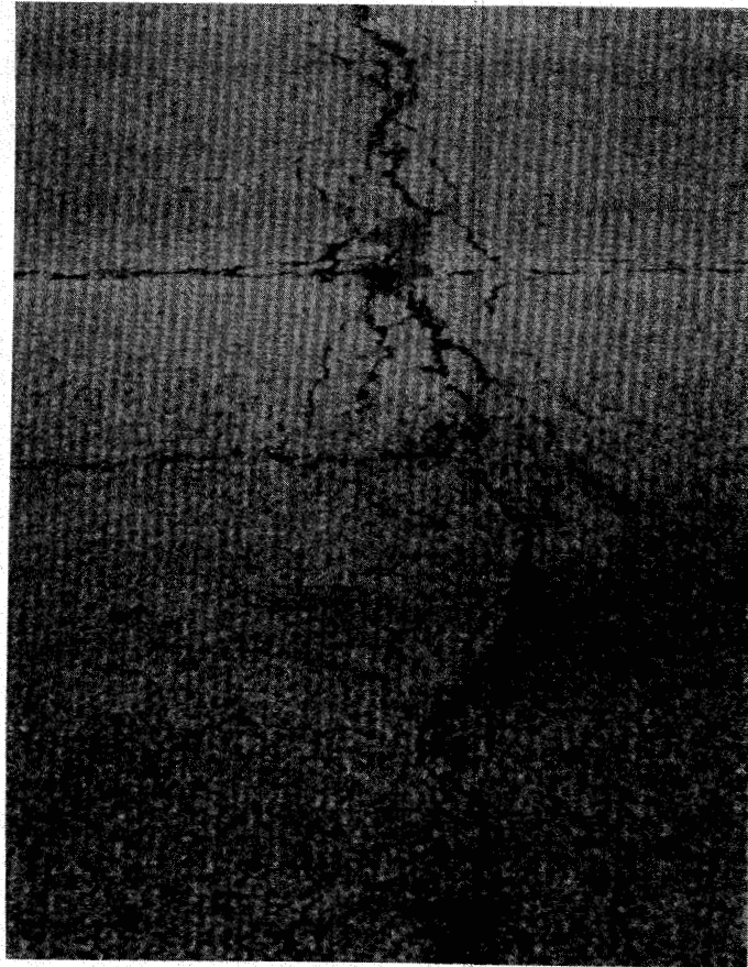
Figure 37. Pavement candidate for crack repair.
