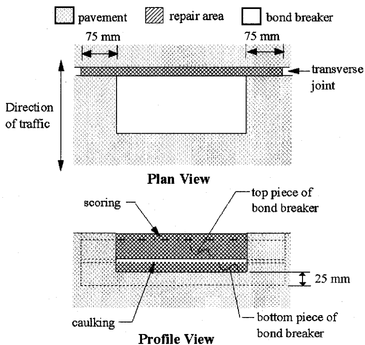
Figure 4-10. Use of latex caulk for joining multiple pieces of bond breaker.
