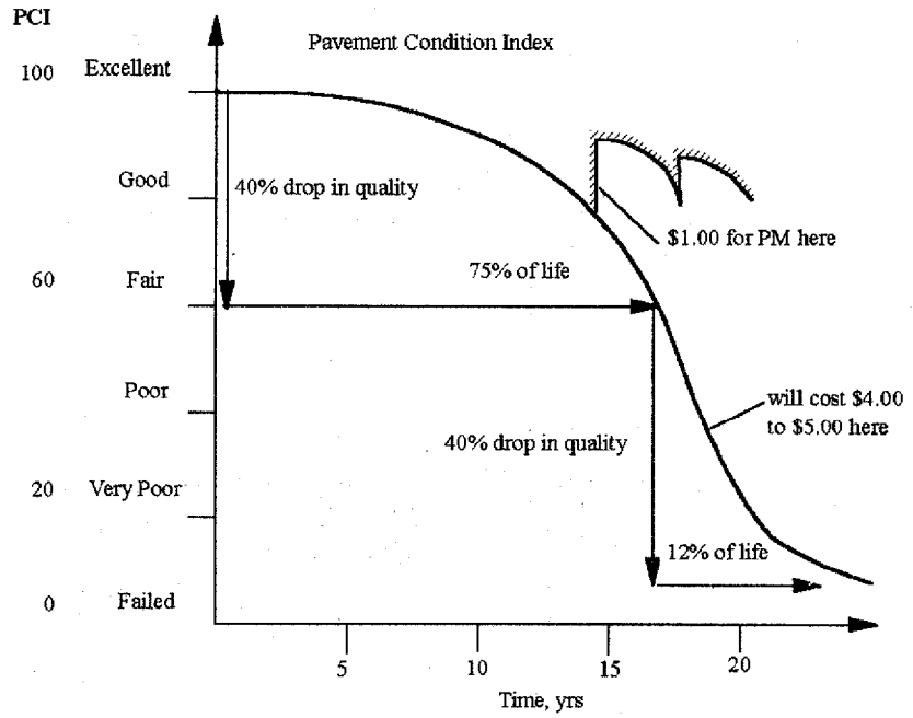
Figure 1-1. Typical pavement life cycle. 1
