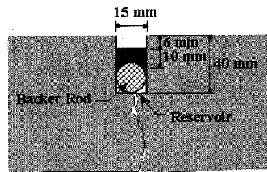
Configuration E Deep Reservoir-and-Recess
