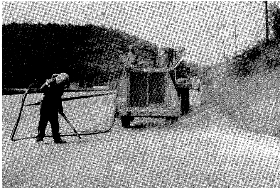
Figure 3-6. Sandblasting operation.
