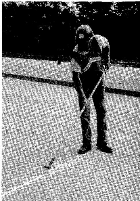
Figure 3-7. Adjustable backer rod insertion tool.
