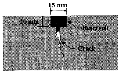
Configuration A Standard Reservoir-and-Flush
