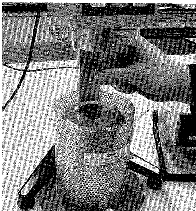
Figure 8. Attaching Spindle Extension with Viscometer Coupling Nut
