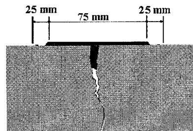
Configuration D Simple Band-Aid
