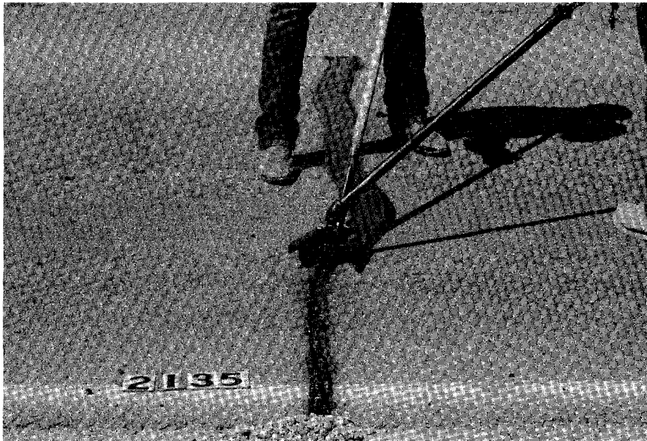
Figure 5-8. Treatment material application.
