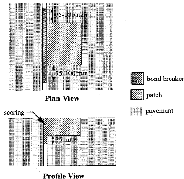
Figure 4-8. Dimensions of joint bond breaker for rigid repairs.
