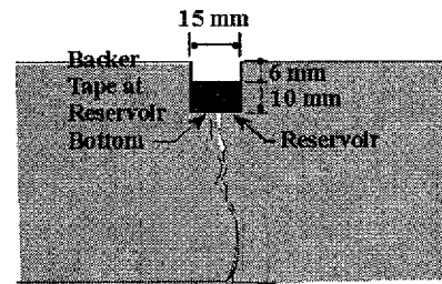
Configuration F Standard Reservoir-and-Recess
