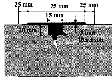
Configuration B Standard Recessed Band-Aid
