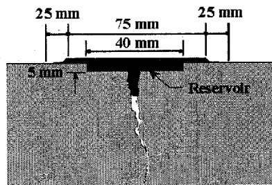
Configuration C Shallow Recessed Band-Aid
