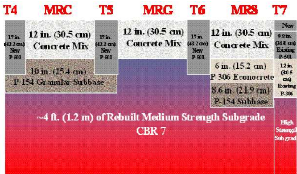
Longitudinal Cross Section of CC-2 Test Items
