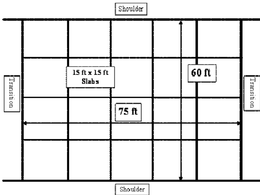
Plan View of Typical CC-2 Test Item Concrete Layer
