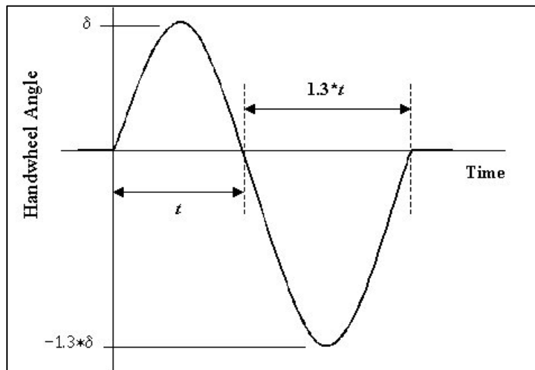
Figure 3. Increasing Amplitude Sine handwheel inputs.
