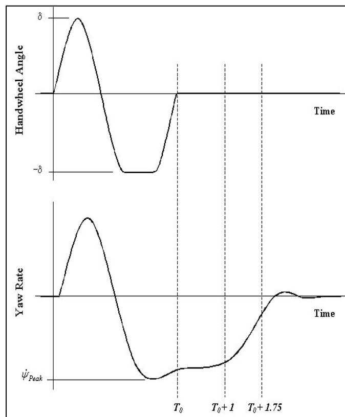
Figure 1. Steering wheel position and yaw velocity information used to assess lateral stability.
