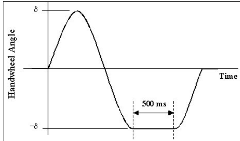
Figure 2. Sine with Dwell handwheel inputs.
