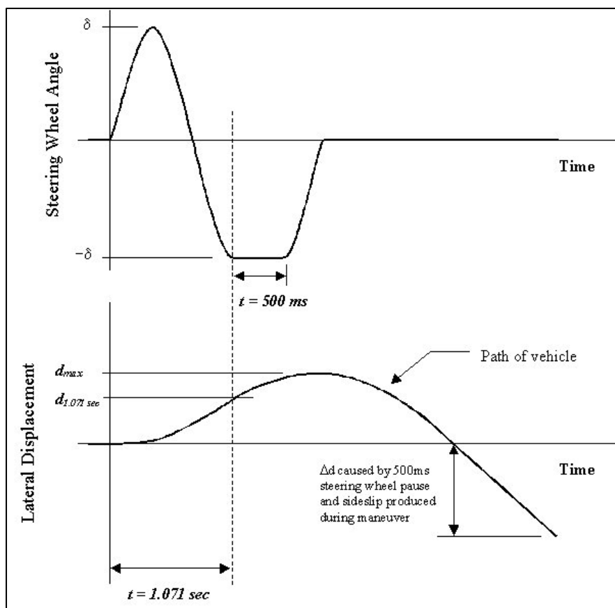
Figure 8. Lateral Displacement in the Sine with Dwell Maneuver
