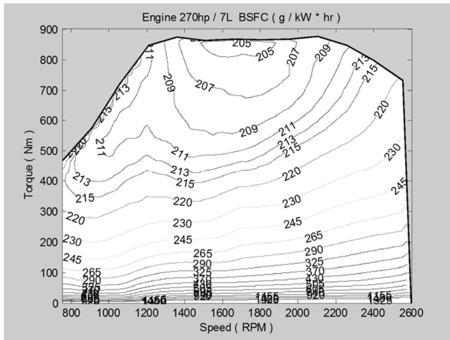
Figure II.5 2018 MHD engine fuel map
