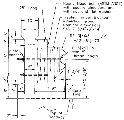
TYPICAL CONCRETE RAIL SECTION WITH W-BEAM RETROFIT WHEN \varnothing 5/8" BOLT CAN NOT GO THROUGH CONCRETE RAILING VOID
