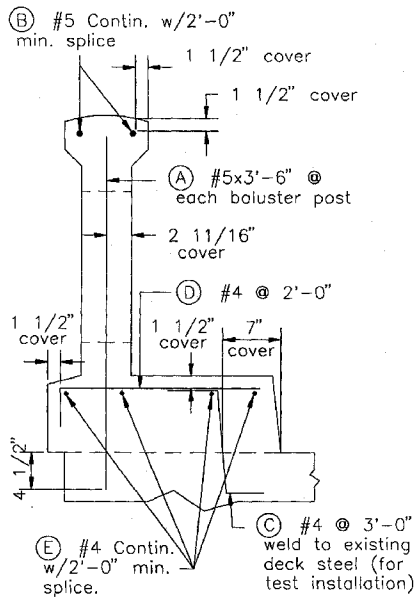
TYPICAL CONCRETE RAIL SECTION REINFORCING
