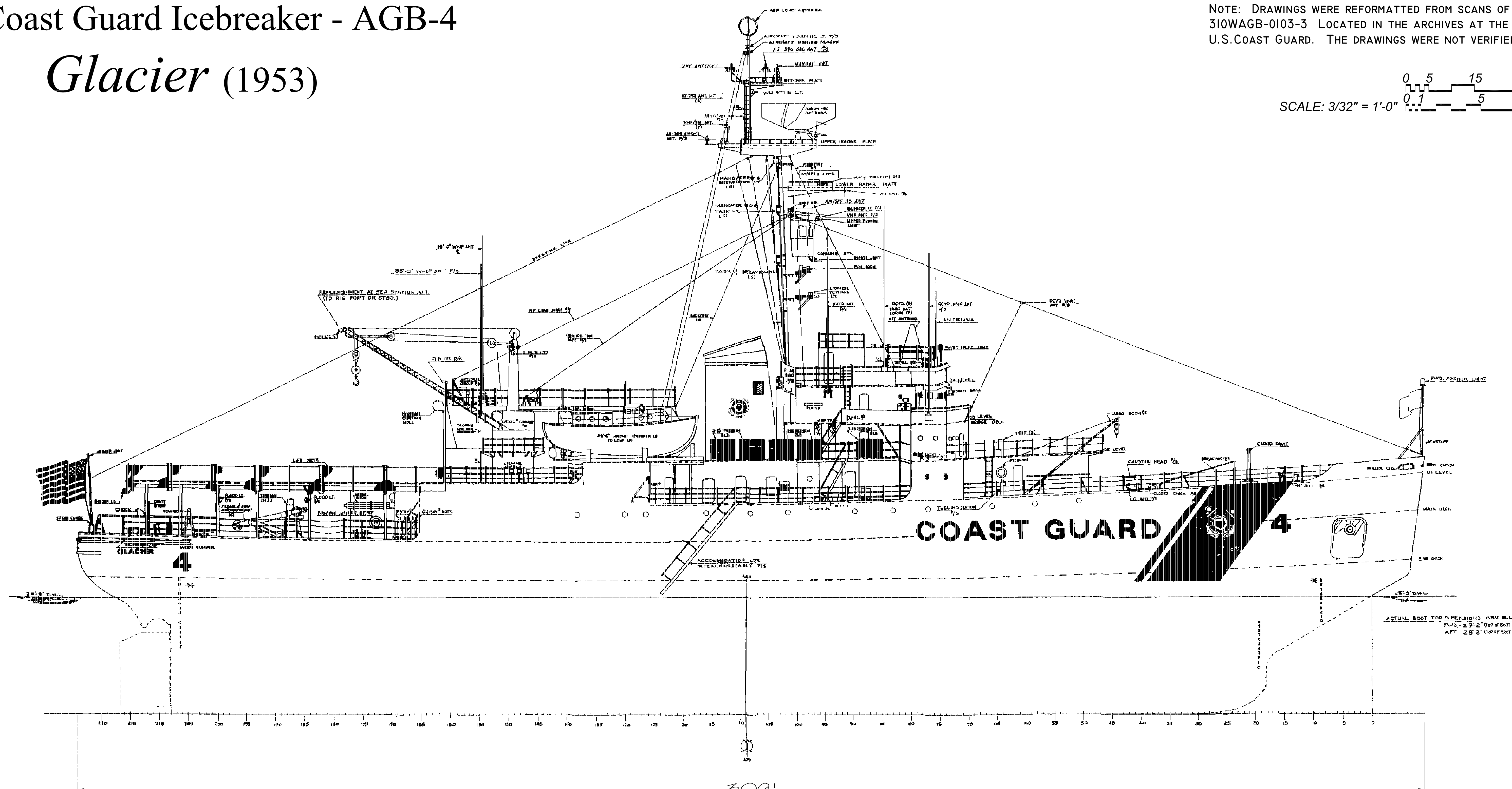
309' PROFILE
