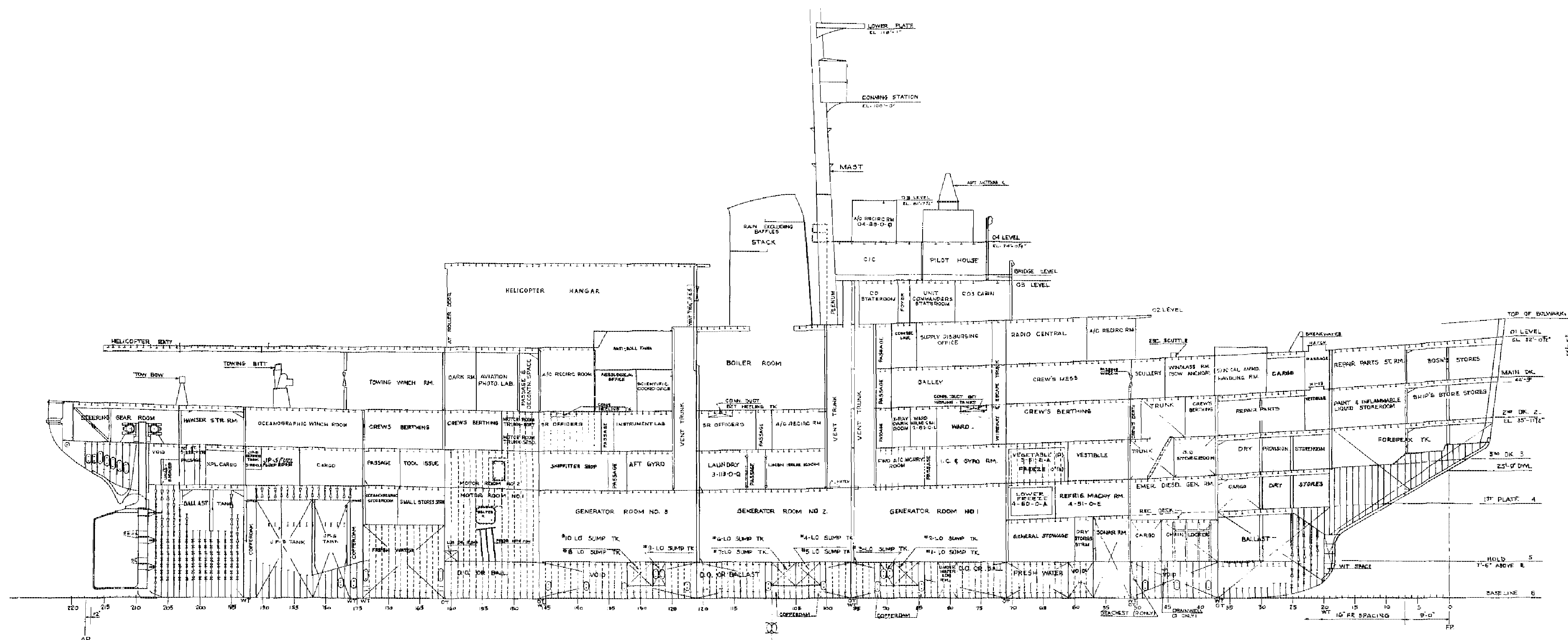
INBOARD PROFILE
