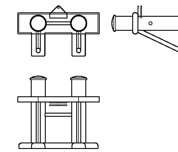
"H" BITT
