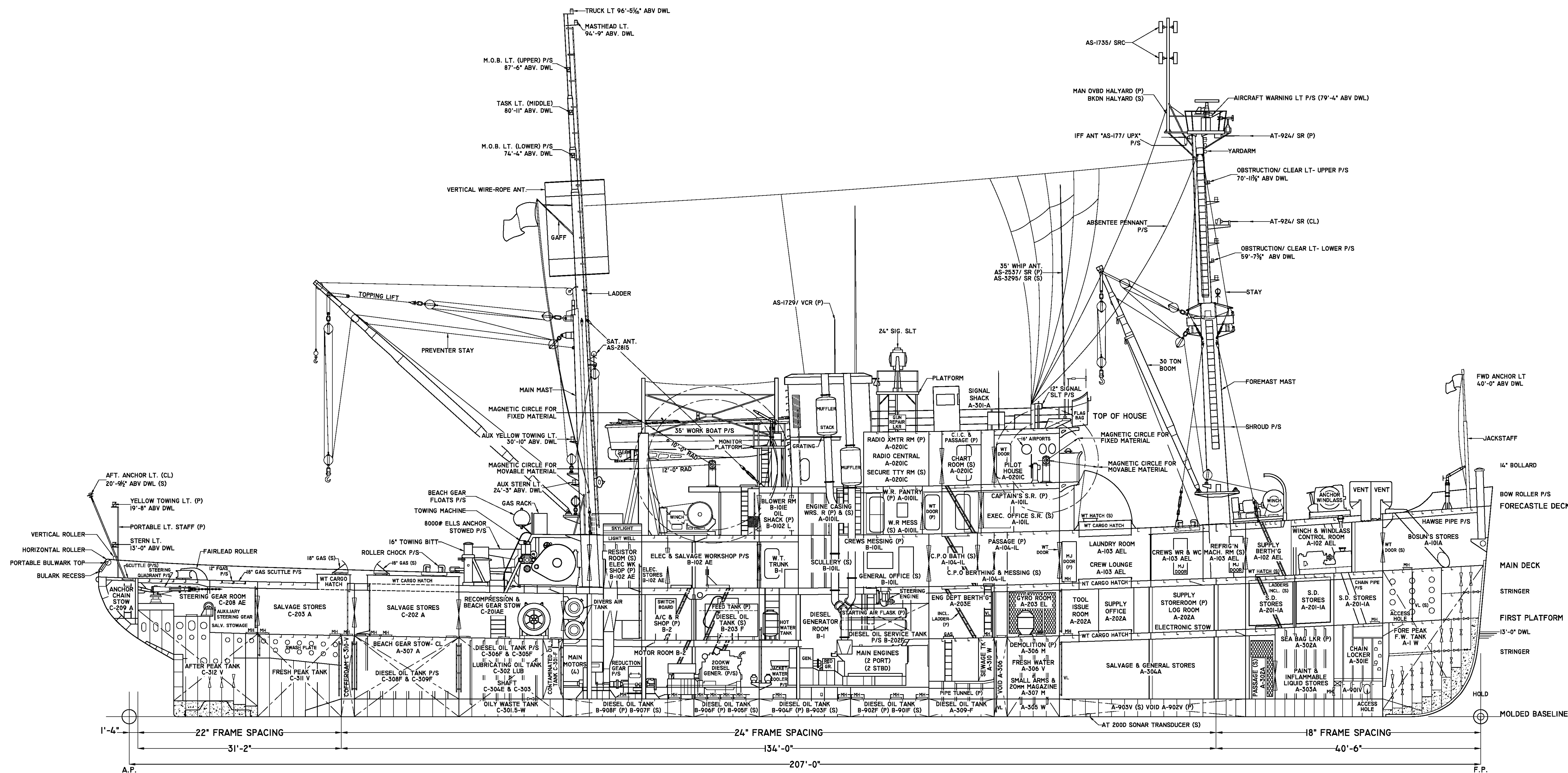
INBOARD PROFILE
