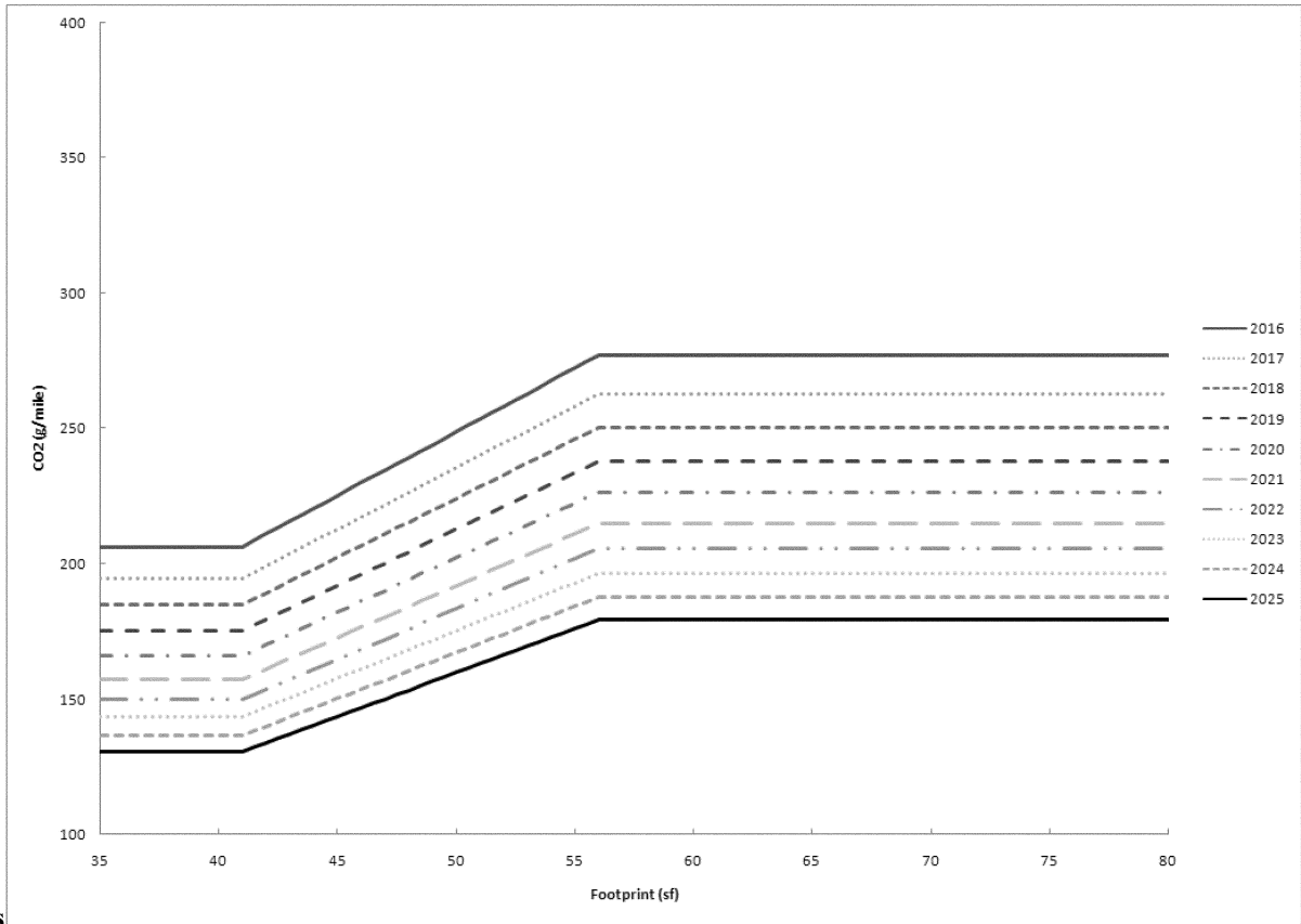
Figure I- 3 CO2 (g/mile) Passenger Car Standards
