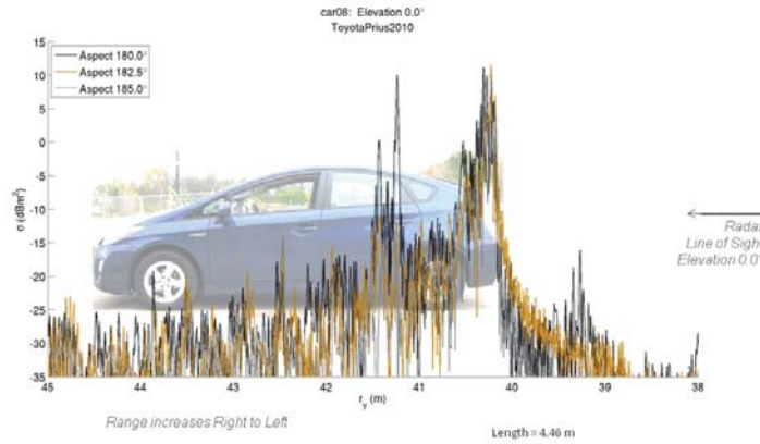
(a) Toyota Prius (2010) returns at 0.0^\circ in elevation
