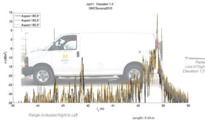
(b) GMC Savana (2010) returns at 1.5^\circ in elevation
