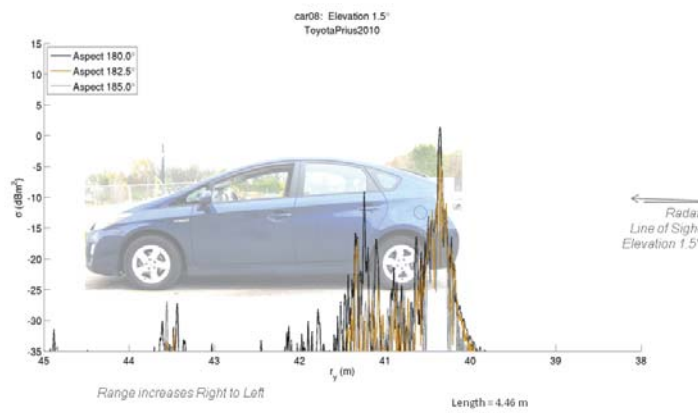
(b) Toyota Prius (2010) returns at 1.5^\circ in elevation
