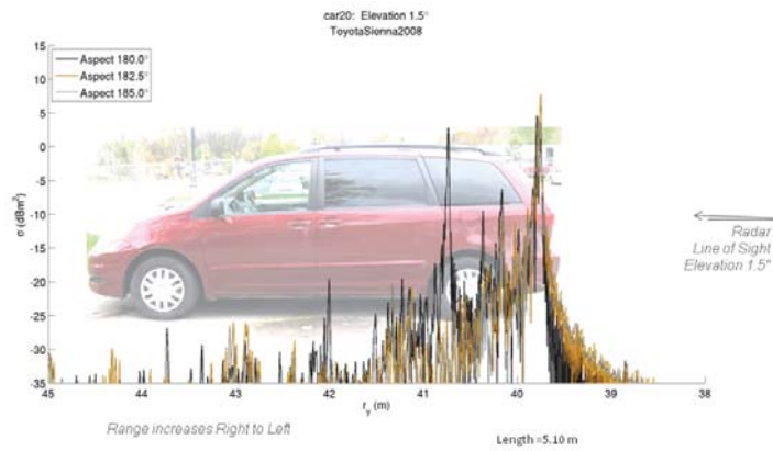
(b) Toyota Sienna (2008) returns at 1.5^\circ in elevation
