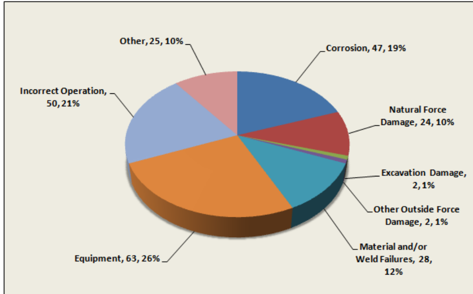
Figure 10: Causes of Significant Onshore Hazardous Liquid Pipeline Incidents Facilities Only (e.g., Pump Stations, Tank Facilities) 2005-2009
