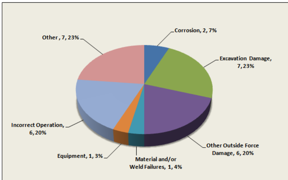
Figure 13: Causes of Onshore Gas Transmission Pipeline Serious Incidents 2005-2009
