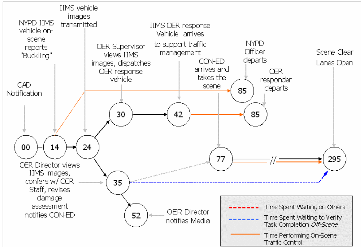
Figure 28. Full IIMS Deployment Activity Network Diagram Incident 2431.
