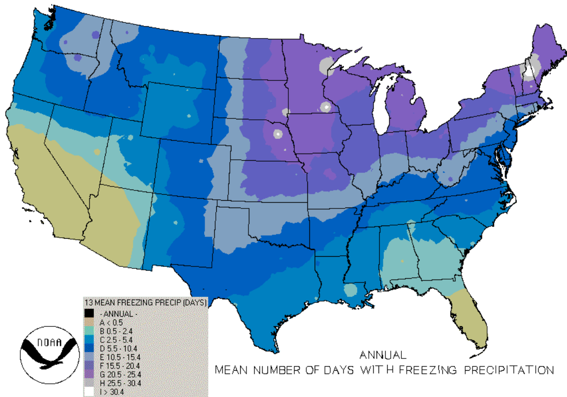
Figure 1. Annual mean number of days with freezing precipitation observed. Source: National Climatic Data Center, 2000.
