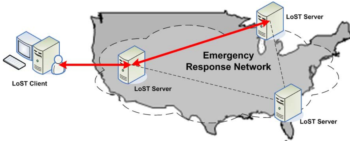
Figure 5.3: LoST Function
