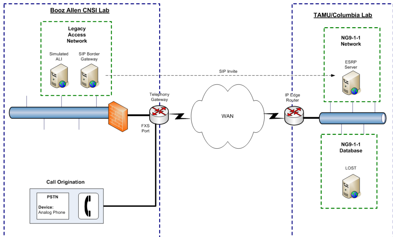
Figure 3.5: Wireline Call Origination Design Overview
