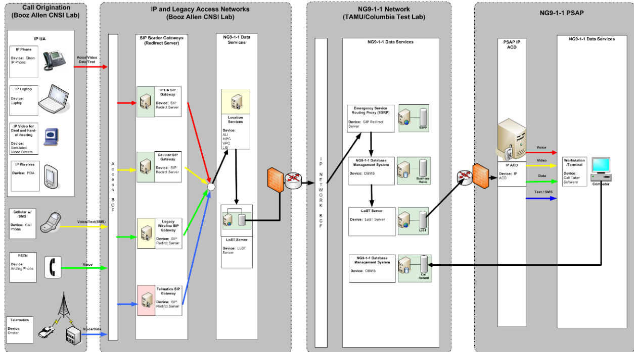
Figure 2.3: Flow Diagram for Call Testing
