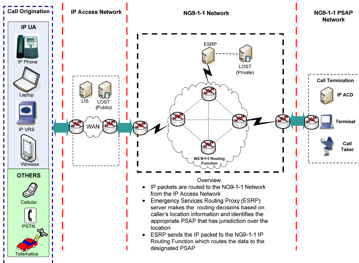
Figure 5.1: NG9-1-1 Network IP Routing Overview
