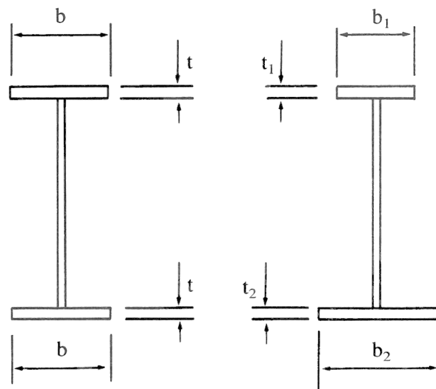
Exhibit 10.4-A GIRDER CLASSIFICATION
