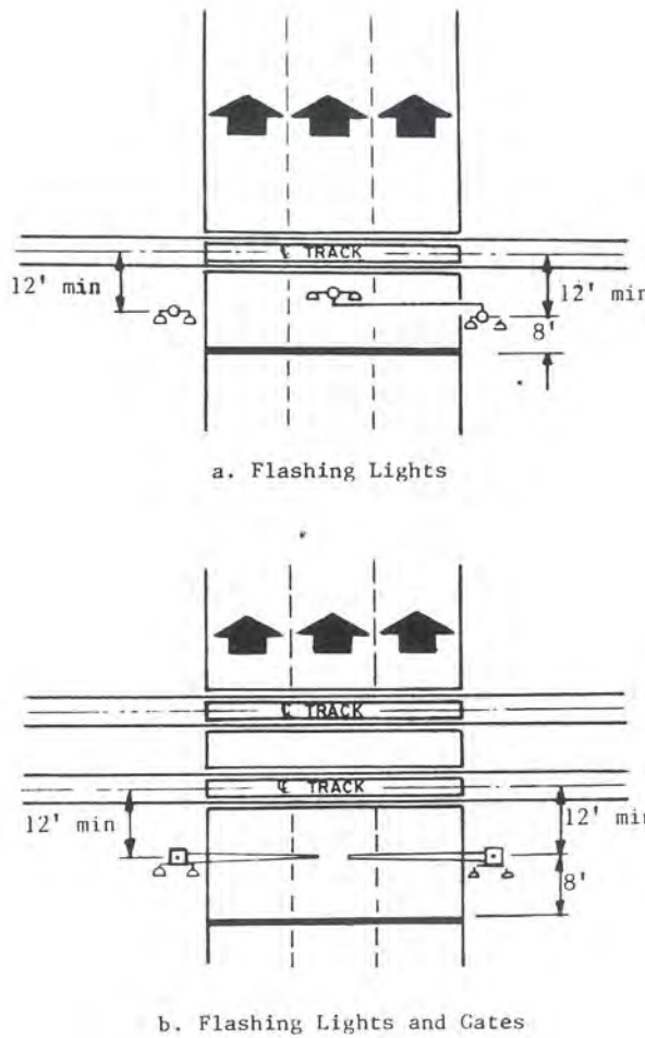
Figure 31. Typical Location Plan, Right Angle Crossing, One-Way, Three Lanes
