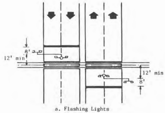
Figure 34. Typical Location Plan, Divided Highway with Insufficient Median for Signals, Two Lanes Each Way
