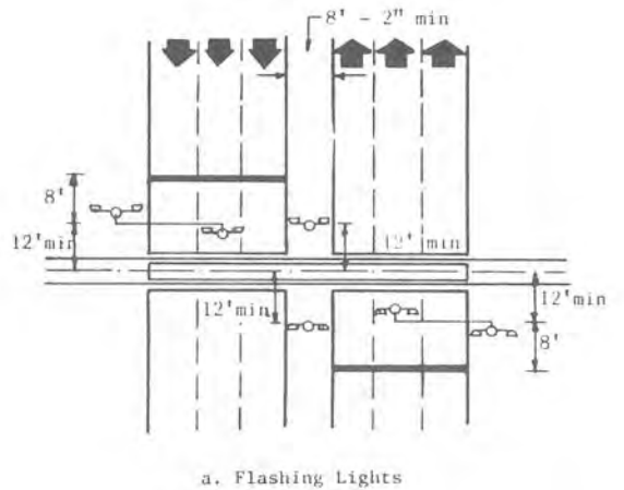
Figure 33. Typical Location Plan, Divided Highway with Signals in Median, Three Lanes Each Way
