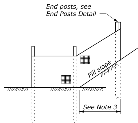
END DETAIL
