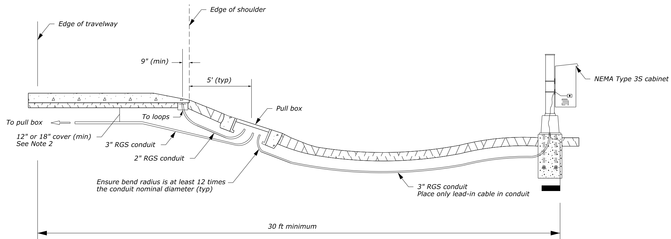
CABINET LOCATION WITHOUT GUARDRAIL OR BARRIER
