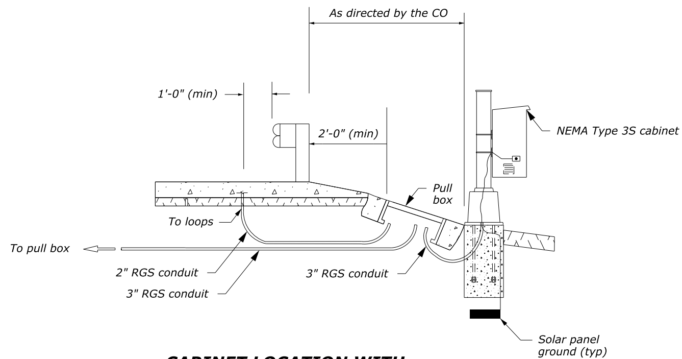
CABINET LOCATION WITH GUARDRAIL OR BARRIER
