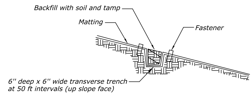
SECTION A-A Erosion Stop (Check Slot) Detail
