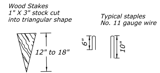
DETAIL A Typical Ground Fasteners
