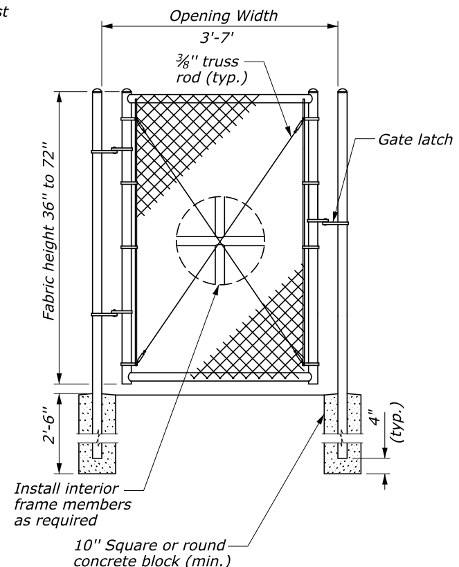
NARROW SINGLE LEAF GATE
