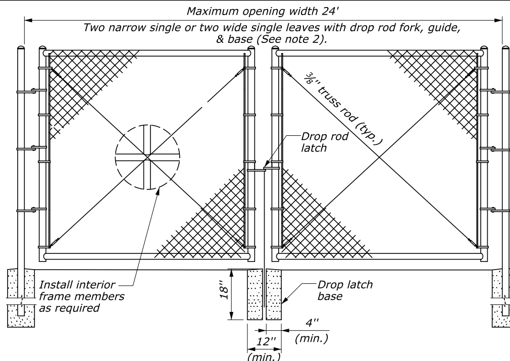
DOUBLE LEAF GATE
