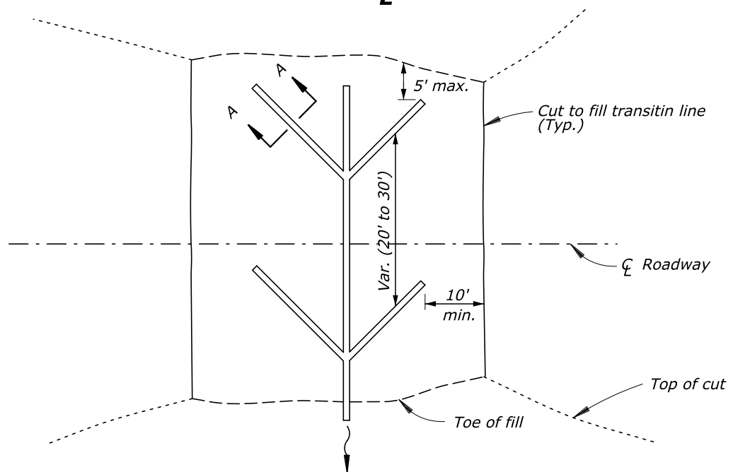
HERRINGBONE DRAINAGE PATTERN (PREPENDICULAR TO \zeta )
