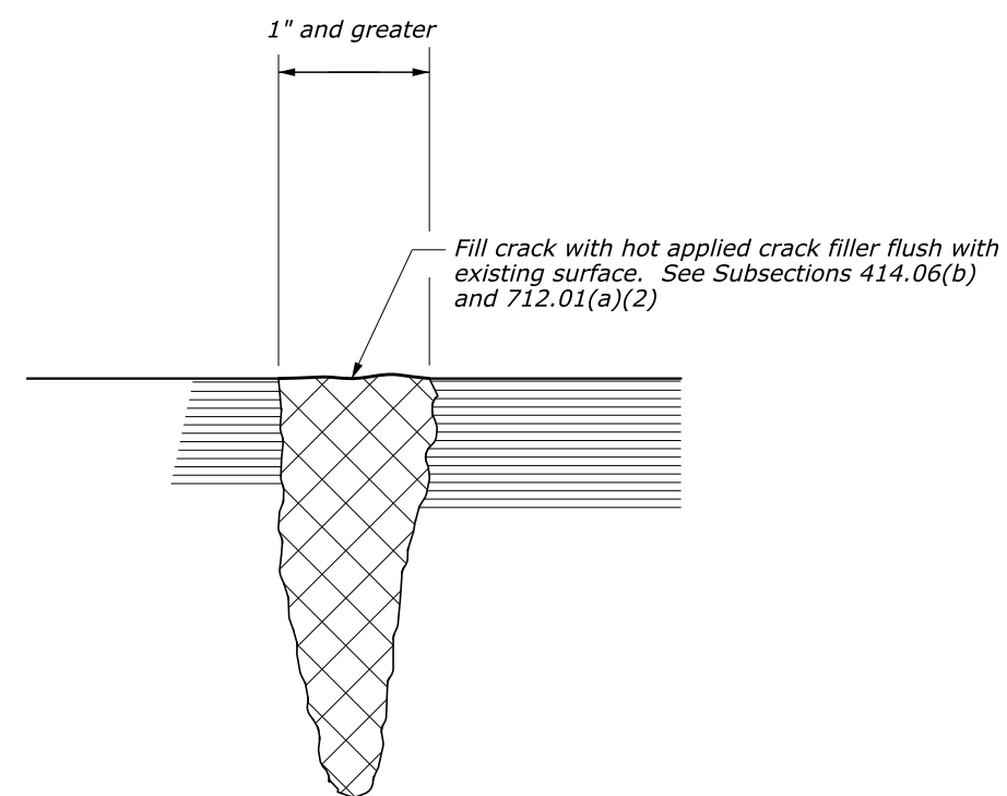
CRACK FILLING
