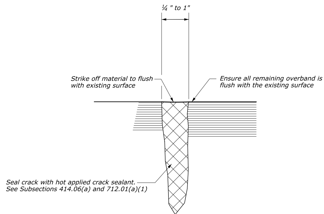
CRACK SEALING
