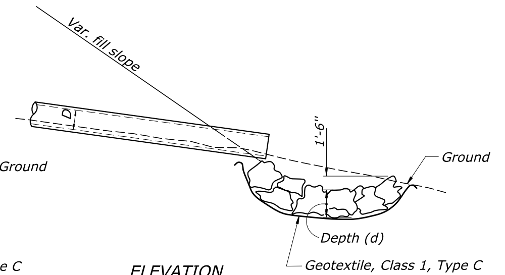
CULVERT WITH NO END TREATMENT
