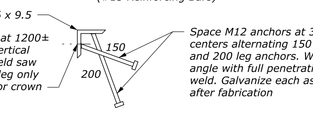
GUARD ANGLE DETAIL (4 required per cattle guard)
