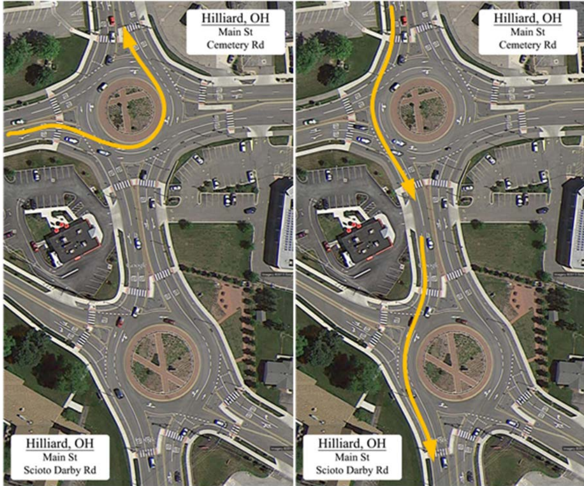
Figure 31. Diagrams. Hilliard, OH, roundabout: Main St. and Cemetery Rd.
