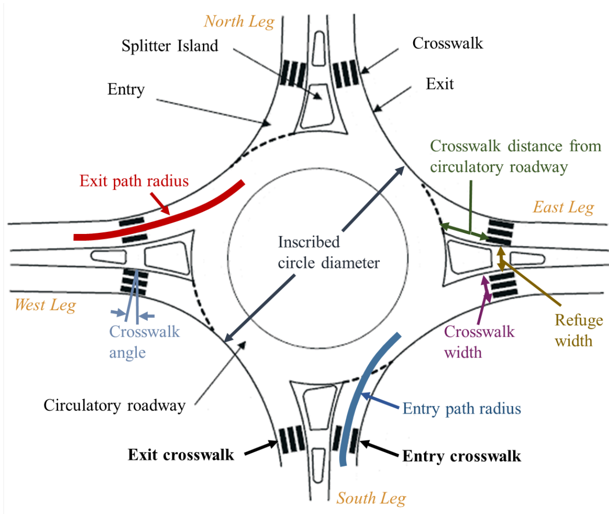
Figure 3. Diagram. Geometric variables for Carmel, IN, roundabout descriptions.
