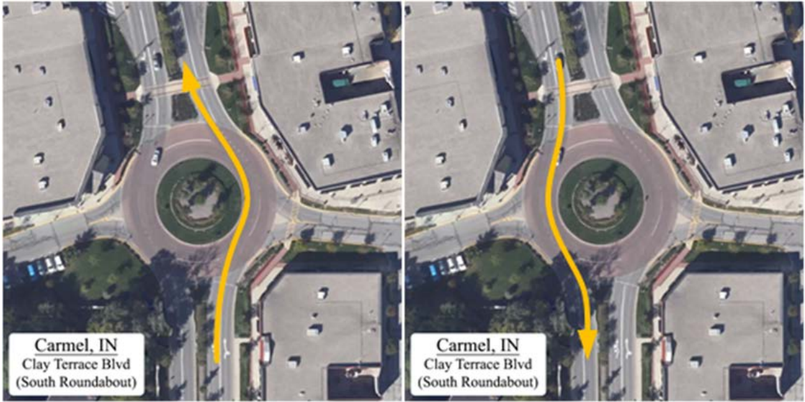
Figure 39. Carmel, IN, roundabout: Clay Terrace Blvd., South Roundabout
