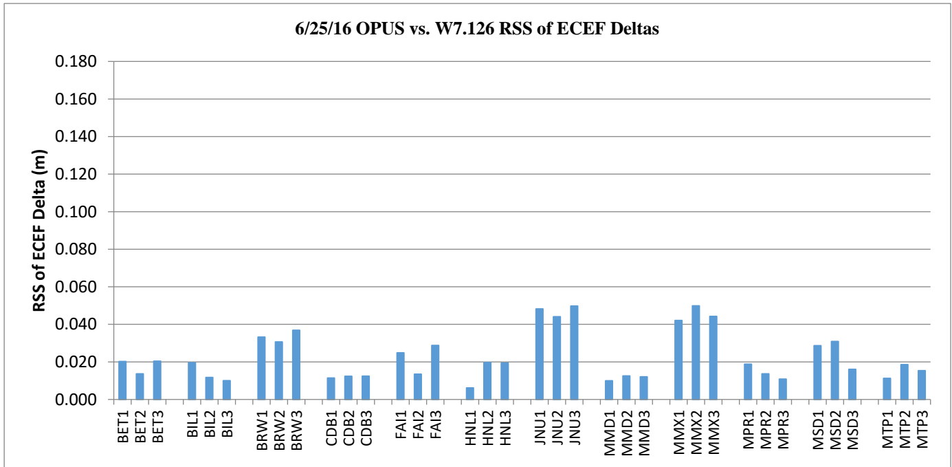
Figure 10-1 Build W7.126 Antenna Positions Deltas OPUS Survey
