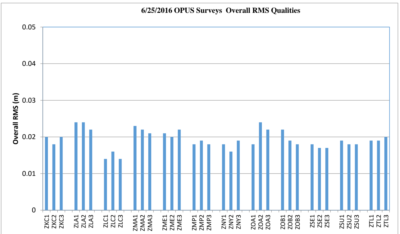
Figure 10-6 OPUS Survey Overall RMS Qualities
