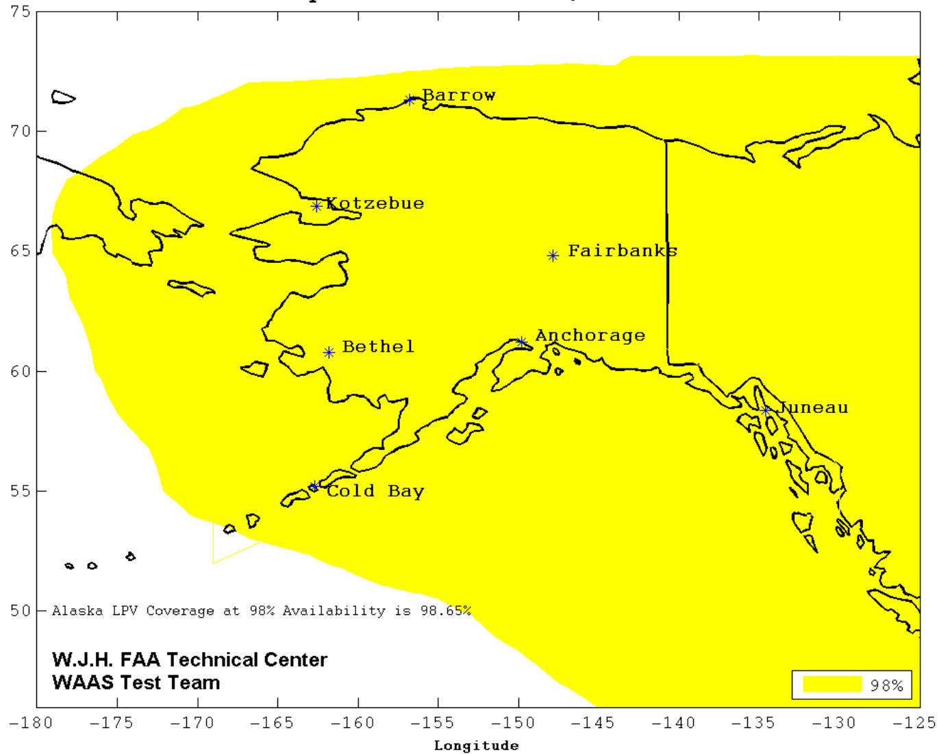
Figure B-4 98% Alaska LPV Availability Contour WAAS 98% LPV Coverage Contours April 1 - June 30, 2016
