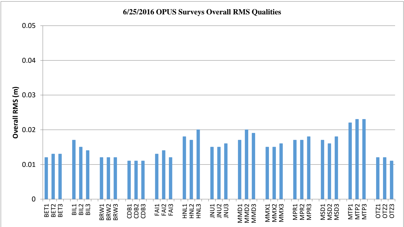
Figure 10-4 OPUS Survey Overall RMS Qualities
