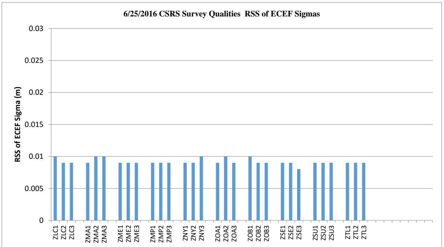
Figure 10-12 CSRS Survey Qualities
