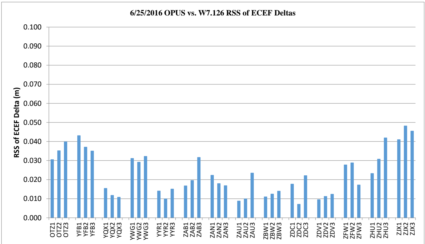
Figure 10-2 Build W7.126 Antenna Positions Deltas OPUS Survey
