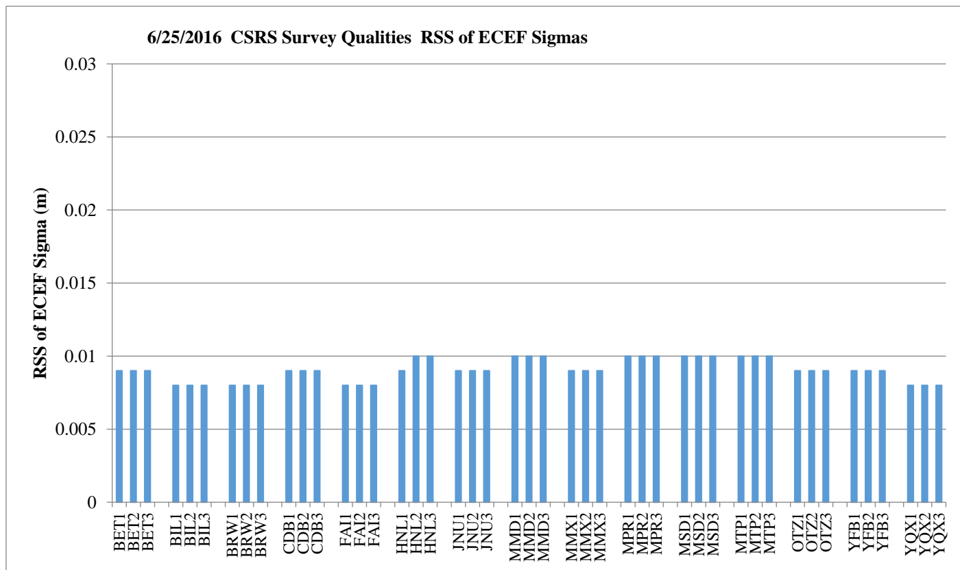
Figure 10-10 CSRS Survey Qualities
