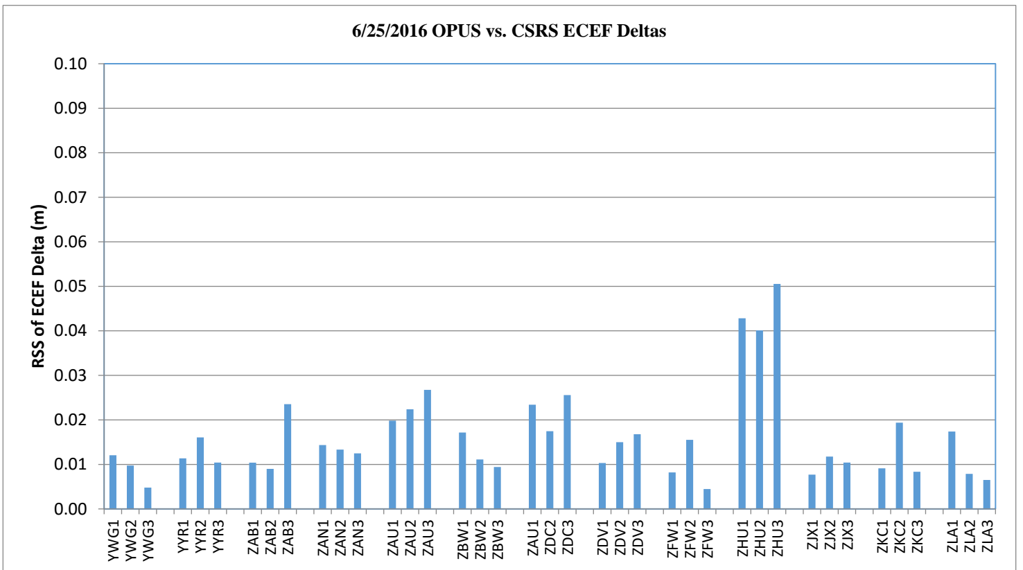
Figure 10-8 OPUS vs. CSRS RSS ECEF Deltas
