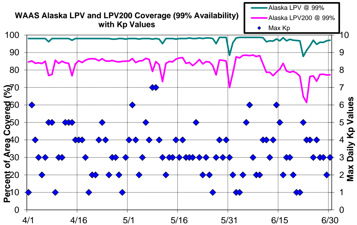
Figure 4-7 Daily LPV and LPV200 Alaska Coverage
