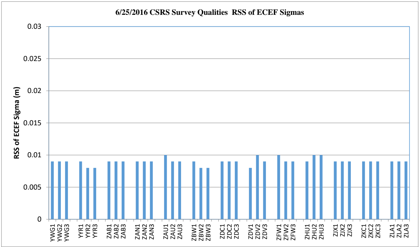
Figure 10-12 CSRS Survey Qualities
