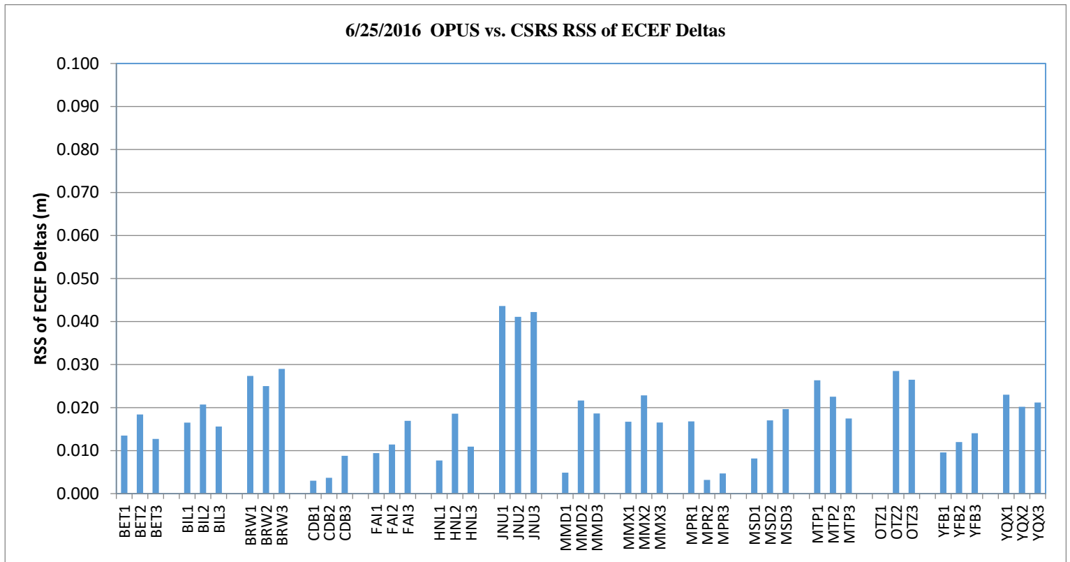
Figure 10-8 OPUS vs. CSRS RSS ECEF Deltas
