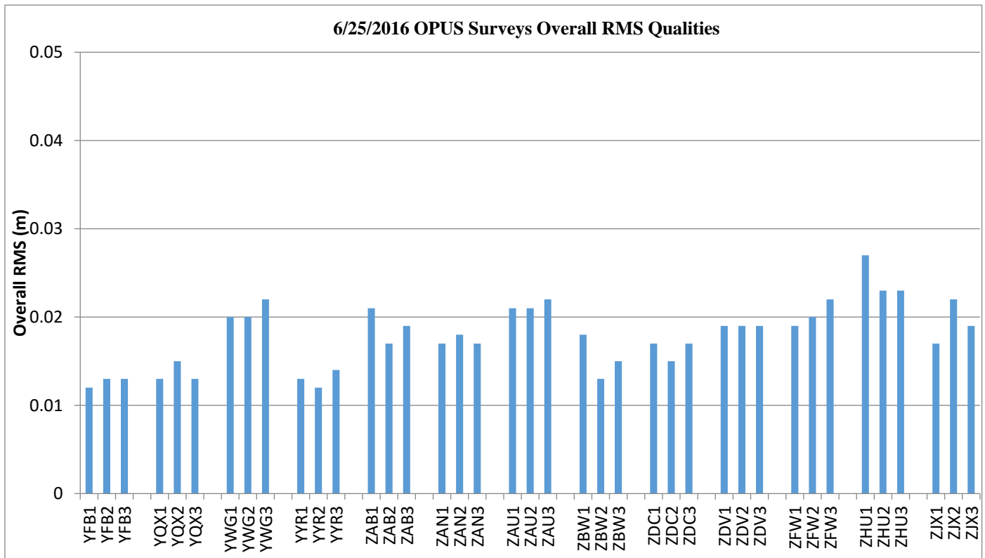
Figure 10-6 OPUS Survey Overall RMS Qualities
