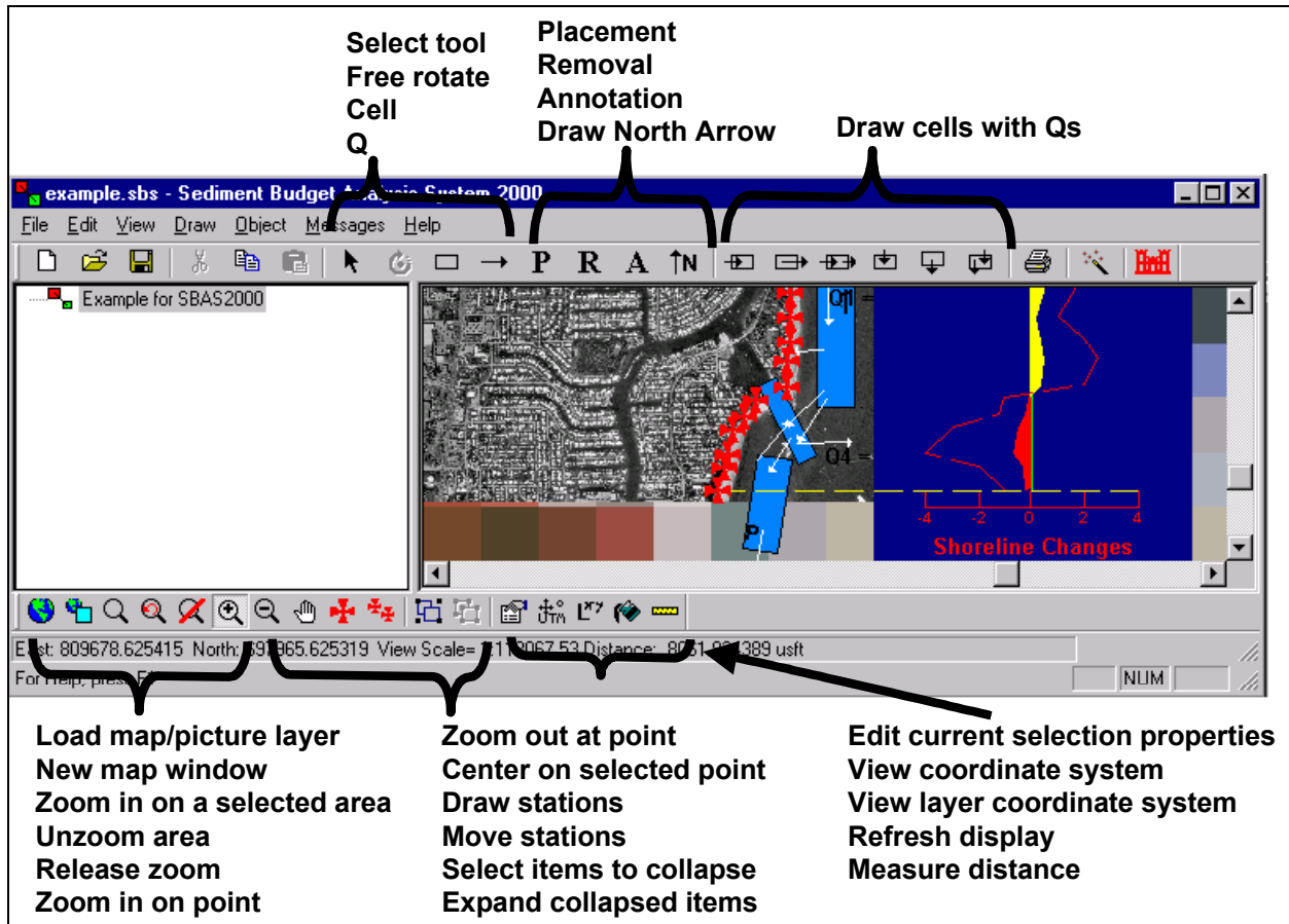
Figure 5. SBAS toolbars and button functions
