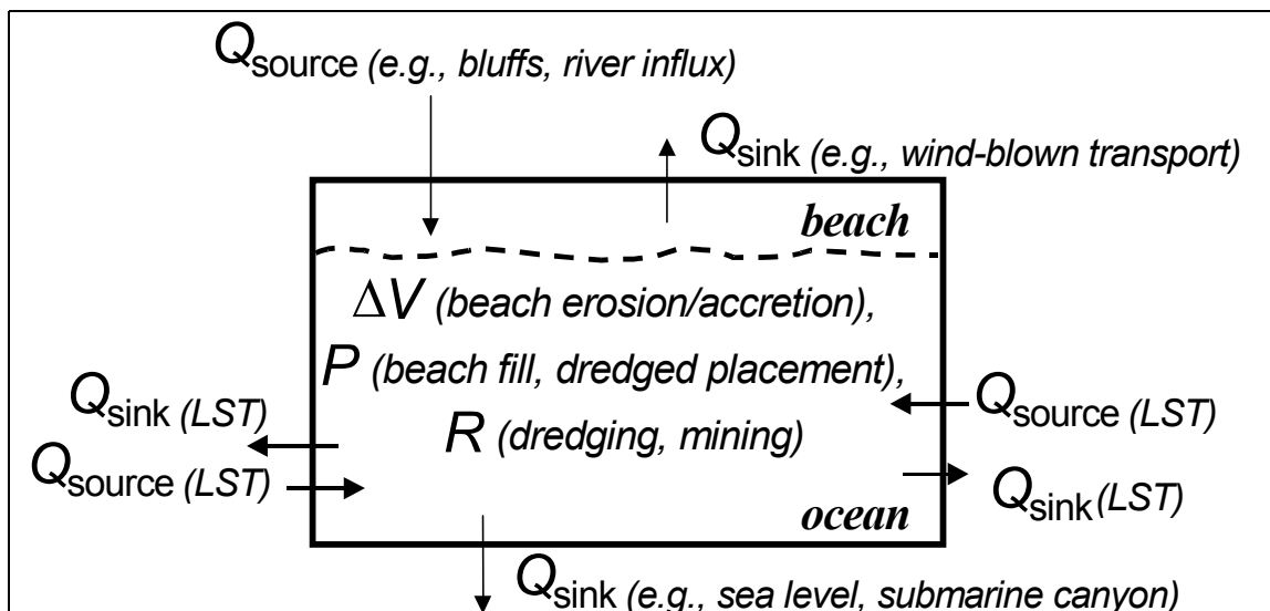
Figure 1. Sediment budget parameters as may enter Equation 1
