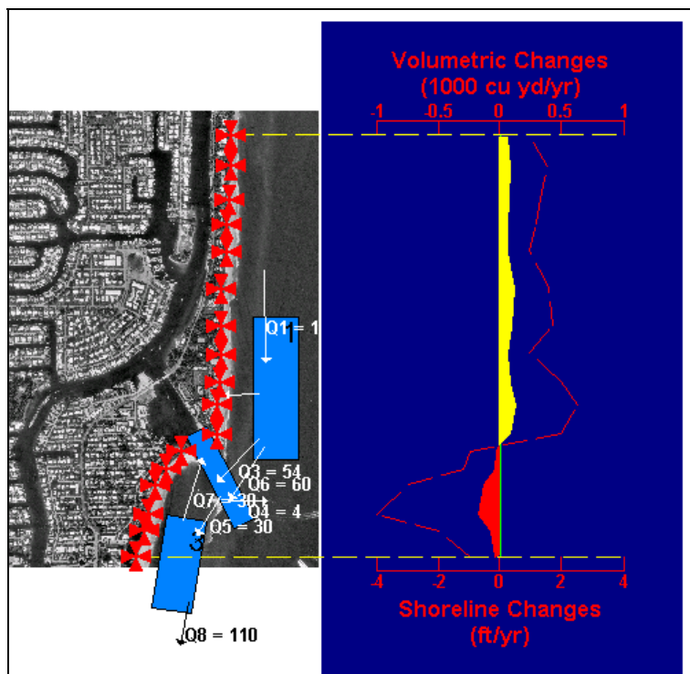
Figure 13. Hypothetical shoreline change data for beaches adjacent to Hillsboro Inlet
