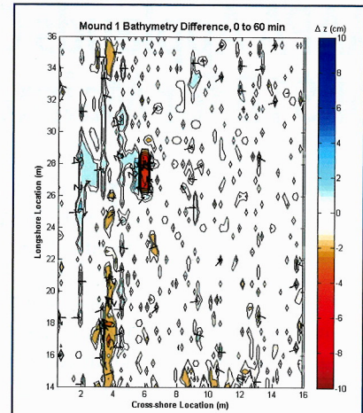
Figure 2: Bathymetry difference after 60 minutes of waves of mound placed at 11-foot depth.
