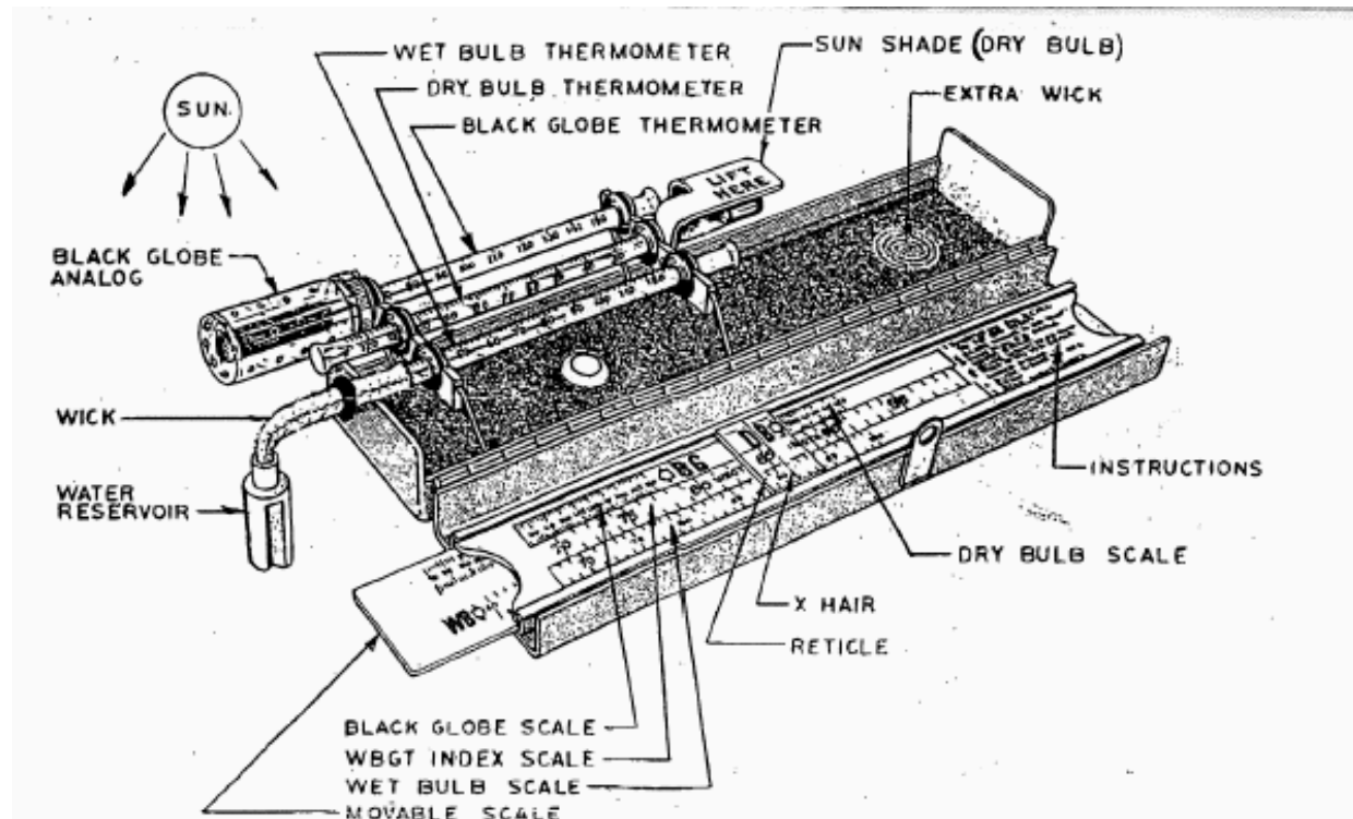
Figure D-1. Wet Bulb Globe Thermometer
