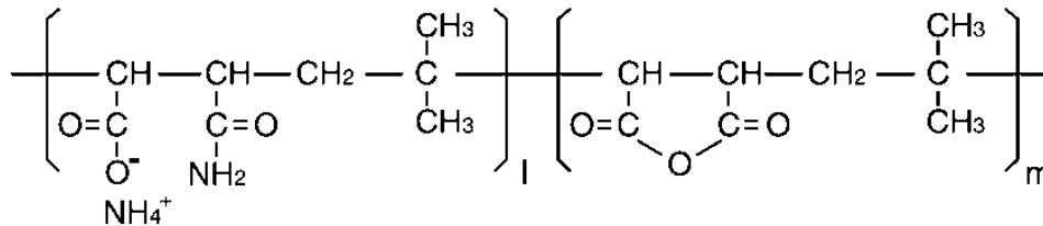
Fig. 1 Molecular structure of the ISOBAM polymer, where l and m represent the 2 types of monomer that alternate linearly along the chain
